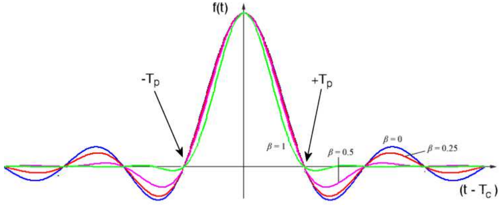
Figure 11: Parameters to define the RaiseCos pulse.
