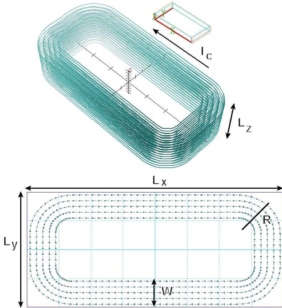
Figure 47: COILBOX with L_x = 4.0 , L_y = 2.0 , L_z = 1.0 , W = 0.5 , R = 0.7 and Ds = 0.1 .
