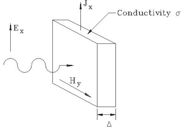
Figure 6: Traveling wave incident on a absorbing layer.
