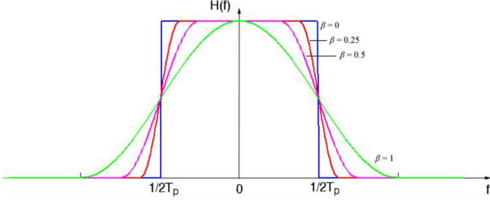
Figure 12: Frequency spectrum of the RaiseCos pulse.
