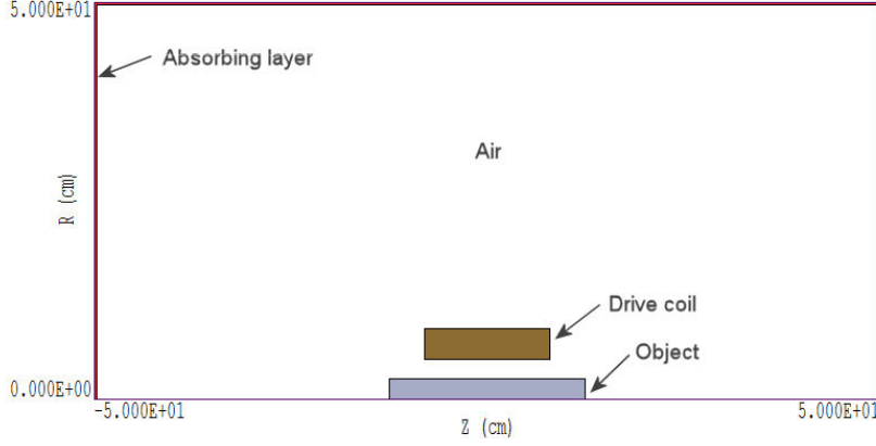
Figure 29: Geometry of example MAGNEAR, dimensions in cm.
