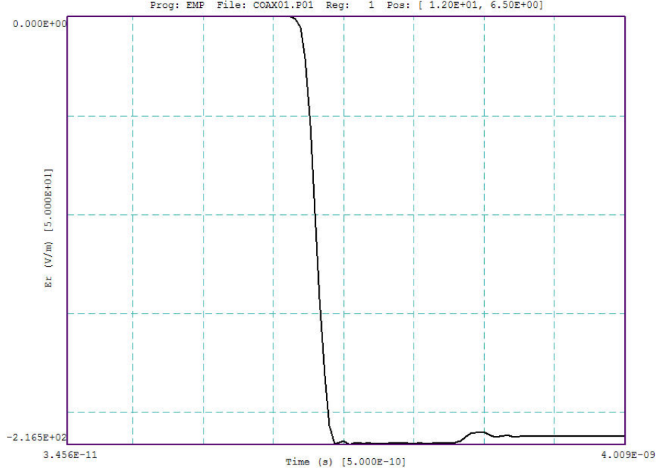
Figure 19: Example COAX01: temporal variation of E_r at position z = 12.0'' , r = 6.5'' .
