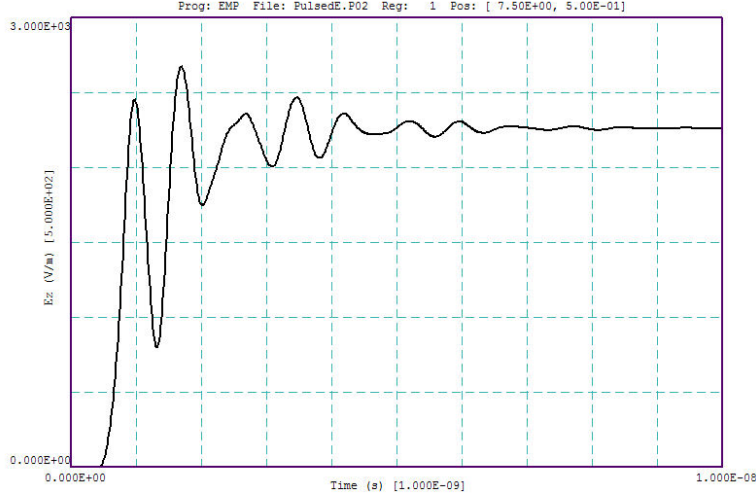
Figure 27: PULSEDE example: calculation of E_z(t) at z = 7.5 mm, r = 0.5 mm.
