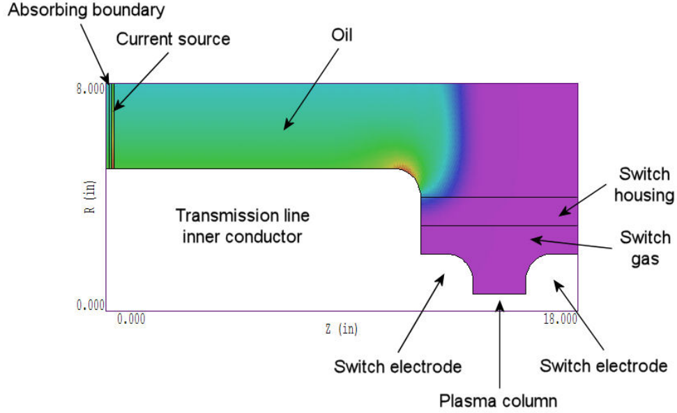
Figure 23: Geometry of the SWITCH example, dimensions in inches. Color code show |\mathbf{E}| at 2.0 ns.
