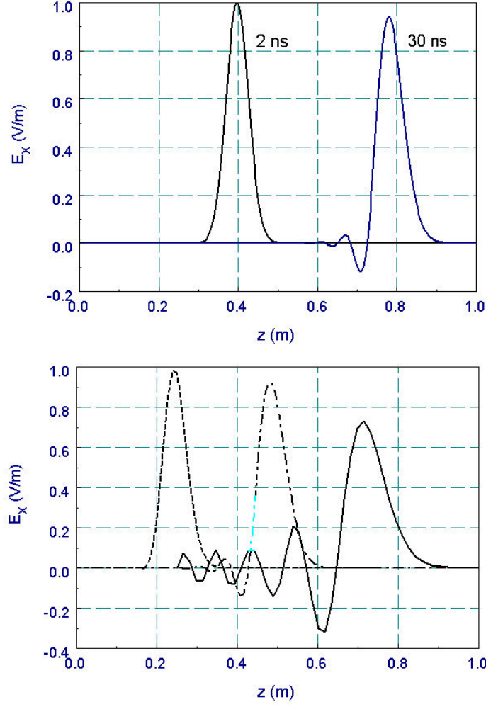
Figure 5: Numerical dispersion in time-domain electromagnetic solution. Gaussian pulse in vacuum, \text{FWHM} = 0.067 m. Top: Pulse shapes after 0.6 and 9.0 m propagation for an element width of 0.004 m. Bottom: Pulse shapes after 2.5 m of propagation as a function of element width. Ratio of pulse width to element width: 16.6 (dotted), 8.3 (dashed) and 4.2 (solid).
