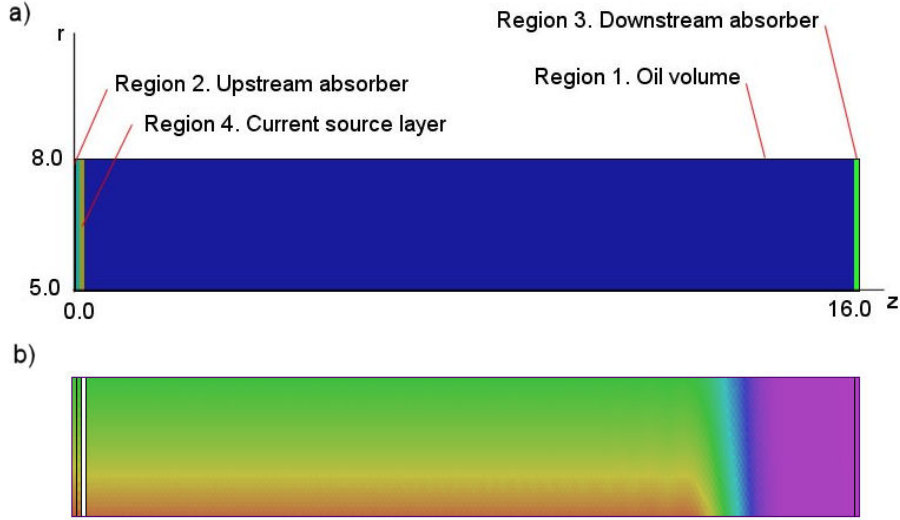
Figure 18: Example COAX01. a) Geometry. b) Distribution of |\mathbf{E}| at 2.0 ns.
