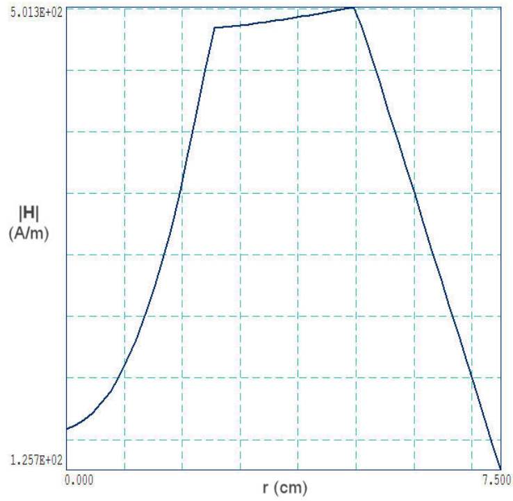
Figure 31: MAGNEAR example: radial variation of |\mathbf{H}| at z = 0.0 cm and t = 3.0 ns.
