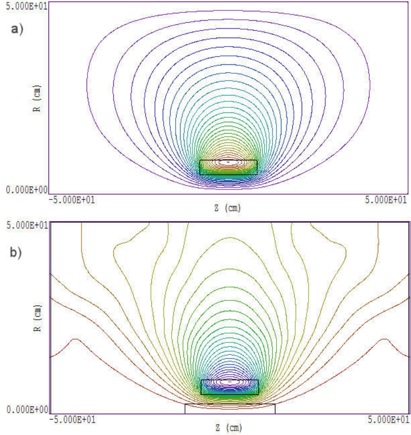
Figure 30: Field line calculations for MAGNEAR example. a) PerMag calculation with 100 A drive. b) EMP calculation at 3.0 ns
