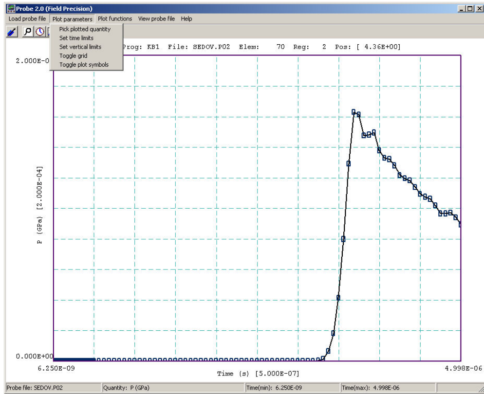
Figure 32: Probe screen shot.
