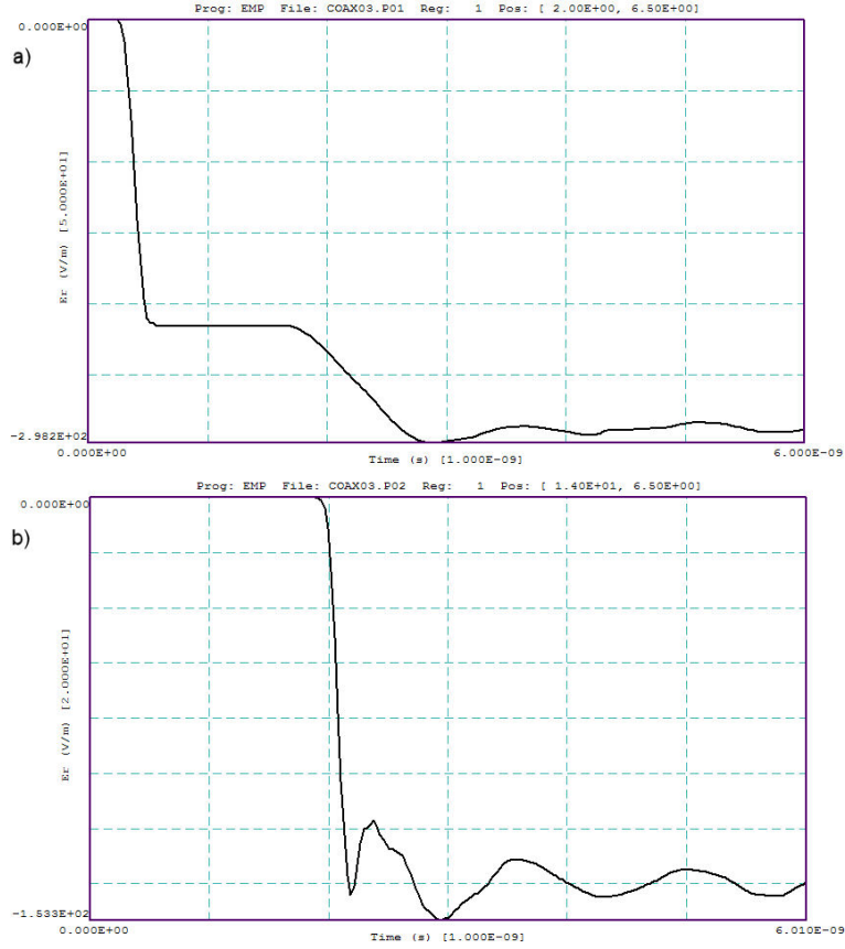
Figure 22: Example COAX03: temporal variation of E_r . a) Position r = 6.5'' , z = 2.0'' . b) Position r = 6.5'' , z = 14.0''
