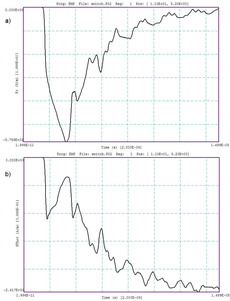
Figure 24: SWITCH example: Probe display of fields measured at the top of the spark gap [ z = 11.0'' , r = 5.2'' ]. a) E_r(t) . b) H_\theta(t) .
