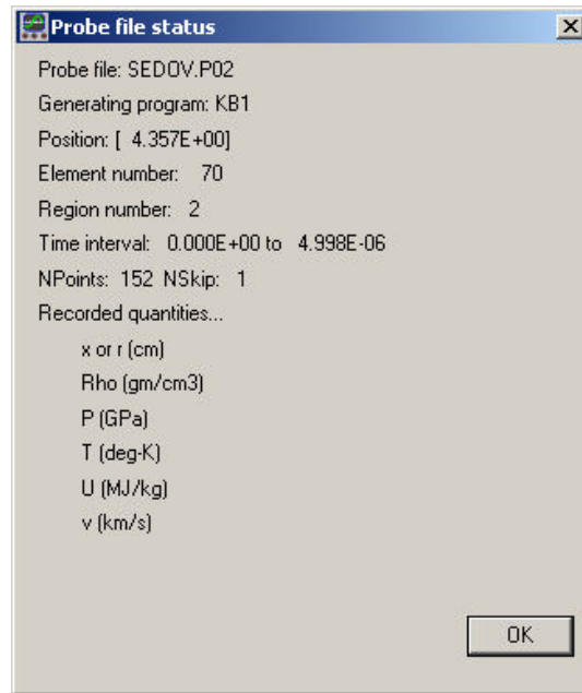
Figure 34: Probe file-information message box.
