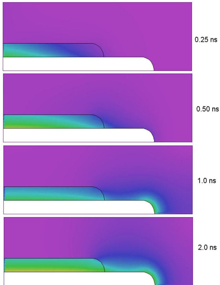
Figure 26: Plots of |\mathbf{E}| for the PULSEDE example.
