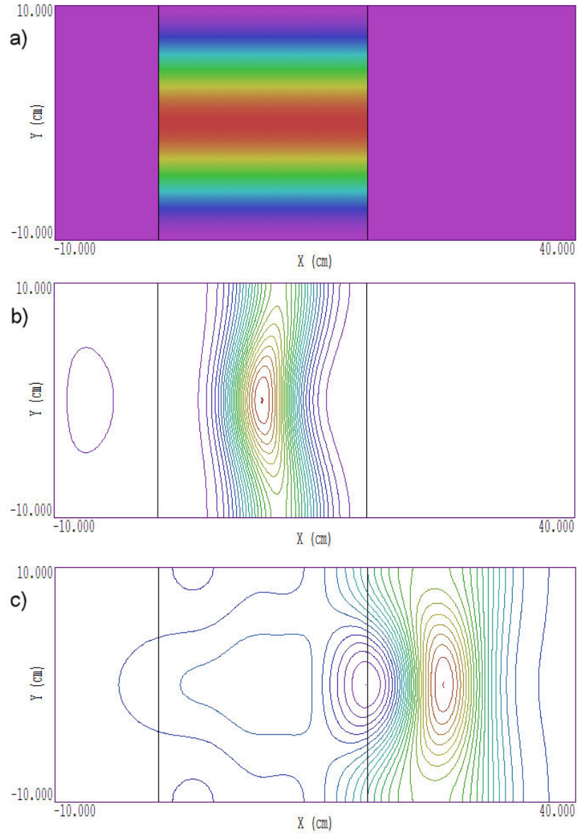
Figure 28: Example GRATING , graded dielectric structure to produce an intensity-modulated plane pulse.
