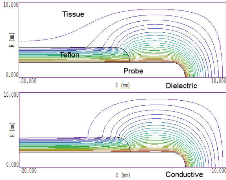
Figure 25: Cylindrical geometry for the EPULSE example, dimensions in mm. a) Equipotential lines for a static solution with ideal dielectrics. b) Equipotential lines for a static solution with ideal conductors.
