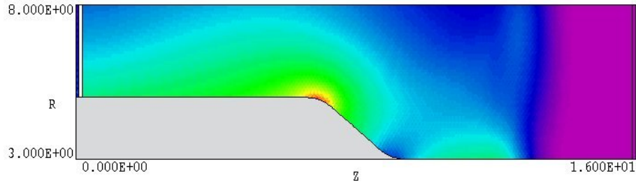
Figure 21: Example COAX03: impedance transition in a coaxial transmission line.
