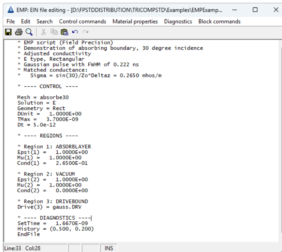
Figure 13: Internal text editor with special functions to create and to modify EMP scripts.
