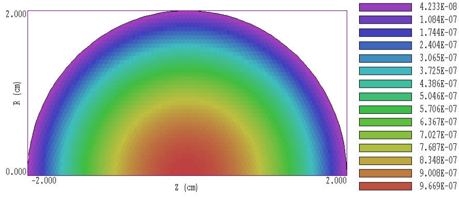
Figure 14: Element plot of \rho(r, z) for the CHARGEFUNC example.
