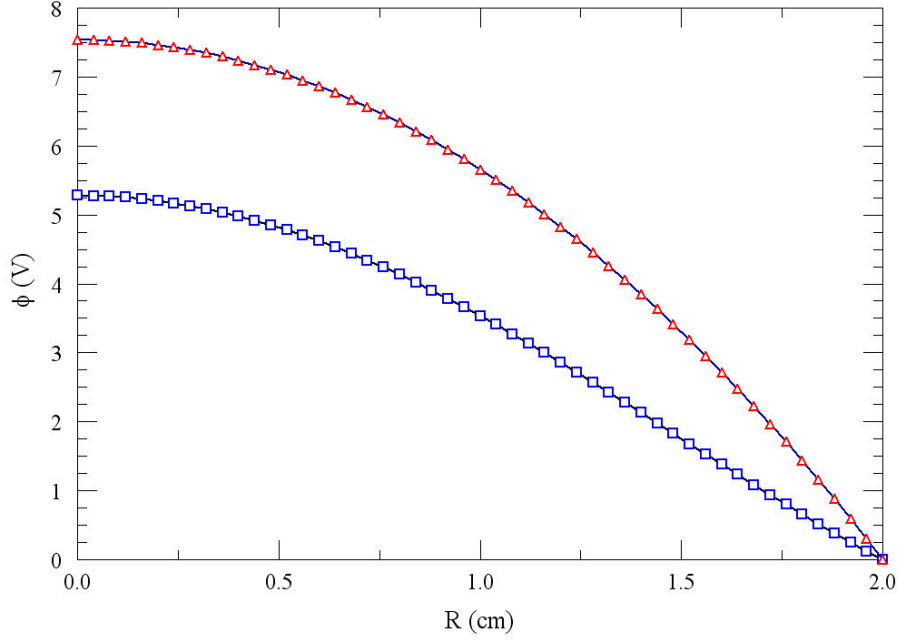
Figure 13: Variation of potential with R for the CHARGEFUNC example. Red: uniform space-charge density. Blue: non-uniform space-charge density.
