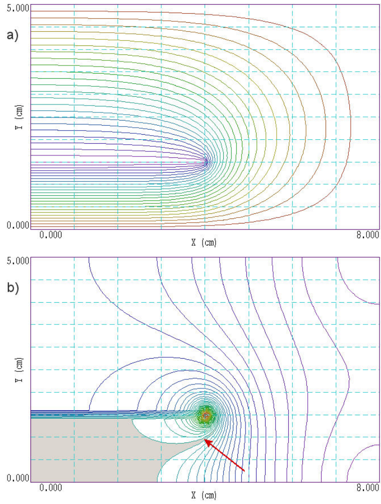
Figure 25: Initial solution, UNIFIELD01. a) Equipotential contours. b) Contours of |\mathbf{E}| .
