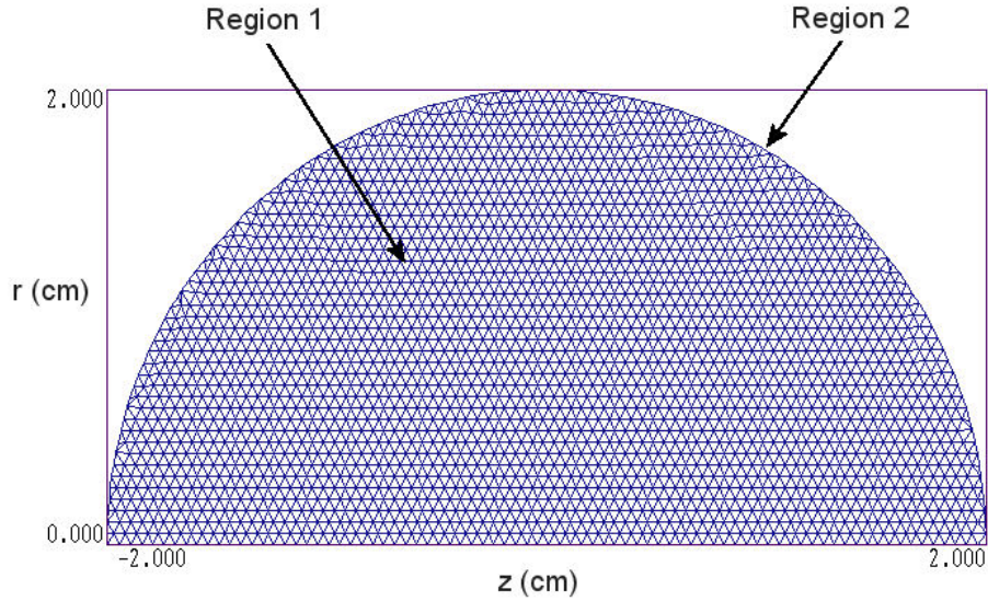
Figure 12: Geometry for the CHARGEFUNC example showing the element size. Dimensions in cm.
