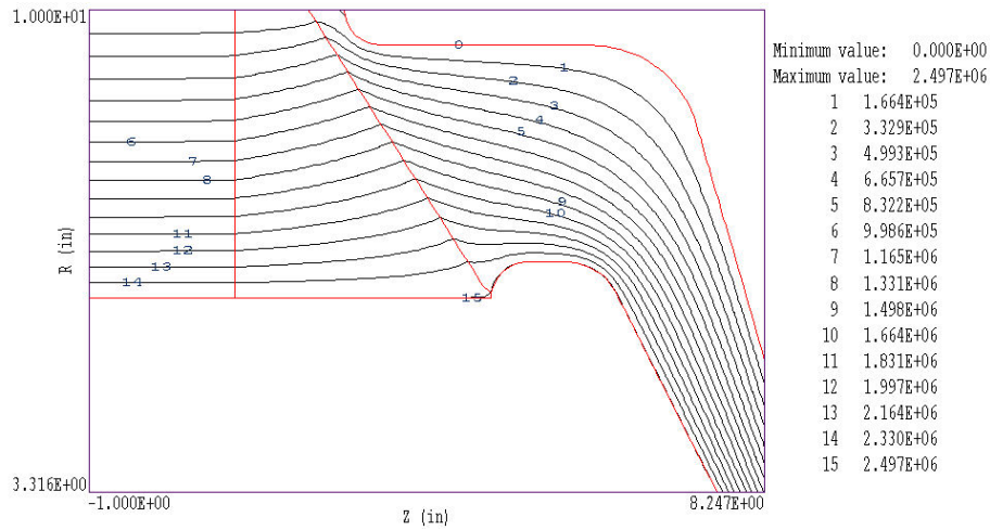
Figure 17: Monochrome contour plot with labels
