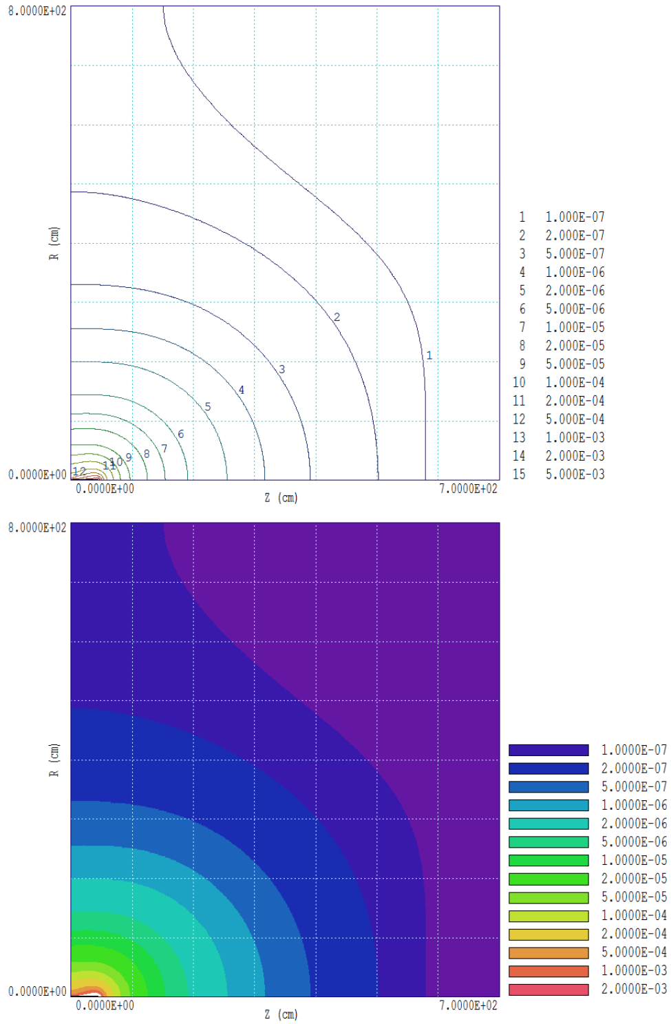
Figure 19: Display of user-specified contour intervals. Top: Contour line plot. Bottom: Filled contour plot.
