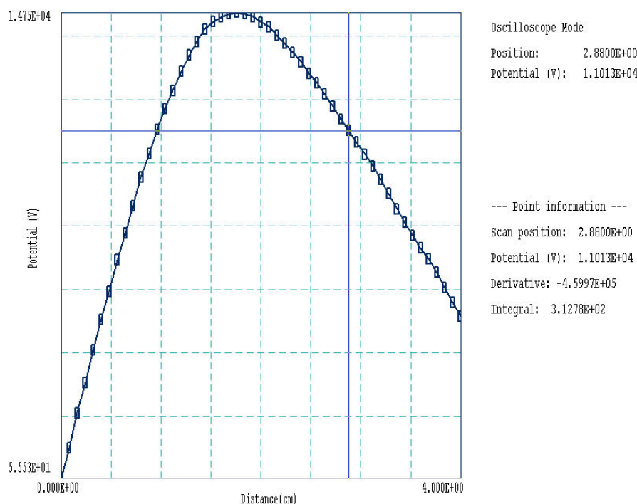
Figure 23: Scan plot in the oscilloscope mode
