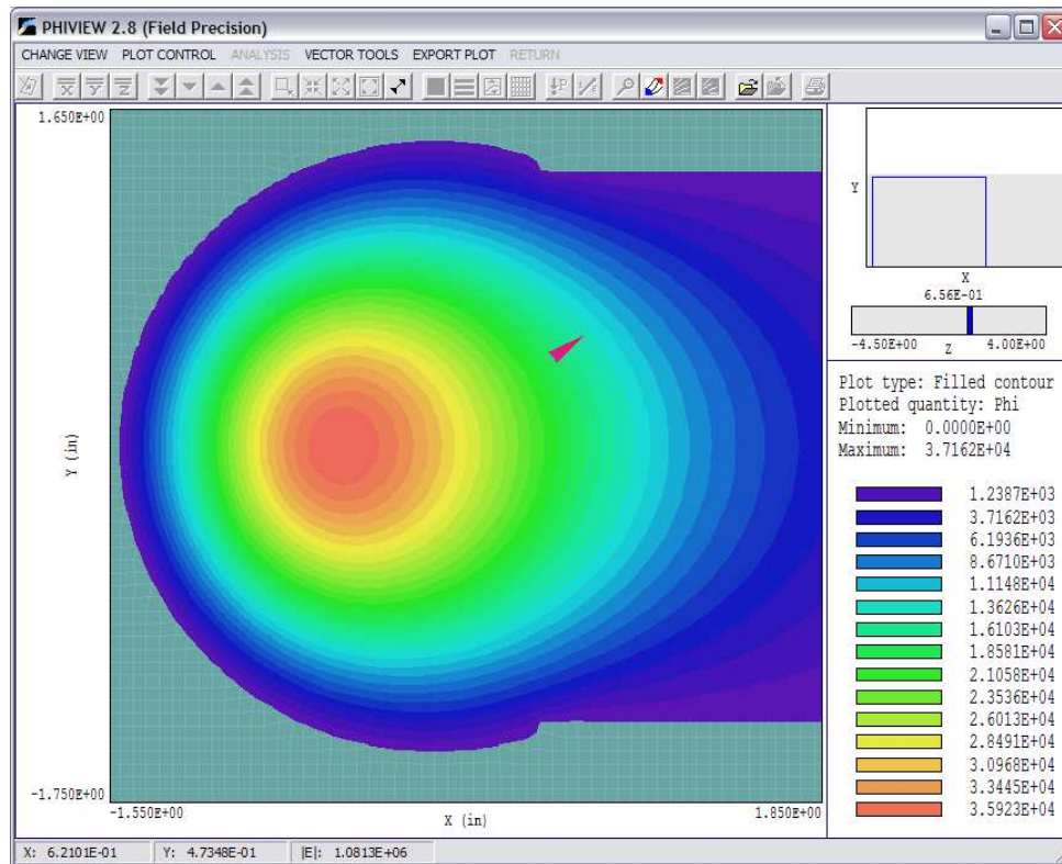
Figure 24: Slice plot – filled-contour plot style.
