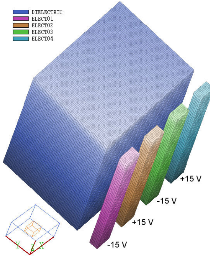
Figure 37: Geometry of example FORCETEST. The diagnostic region is not shown.
