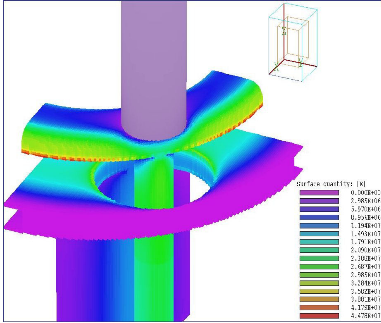
Figure 30: Three-dimensional surface view of region boundaries with color coding by electric field magnitude.
