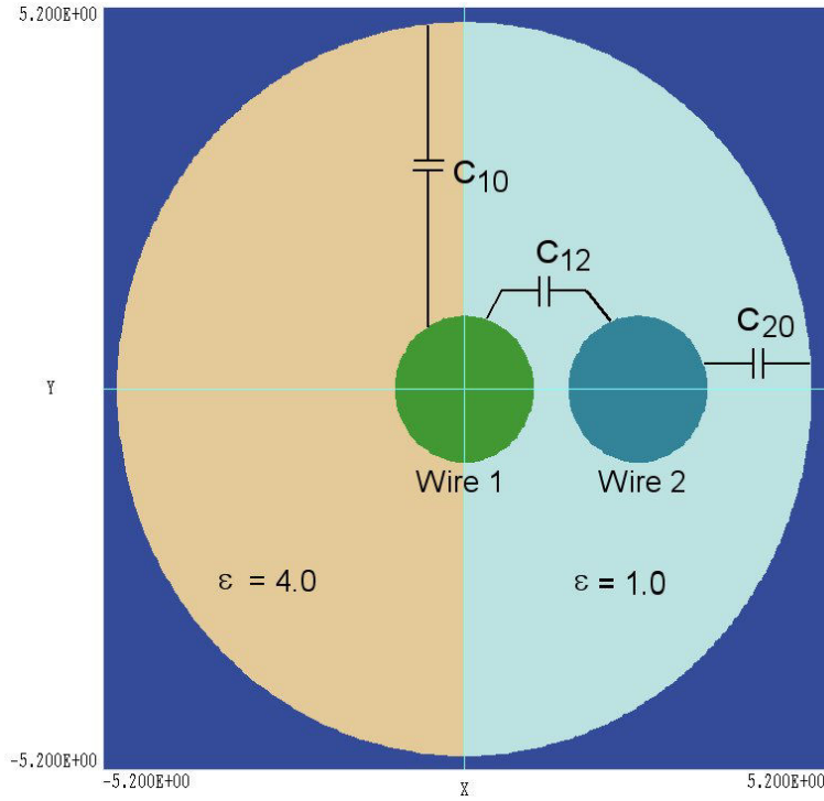
Figure 39: Benchmark example – geometry and definition of quantities (system is uniform in z with a length L_z = 0.02 m).
