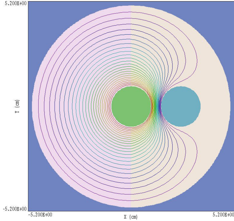
Figure 40: Calculated equipotential lines for Solution 1.
