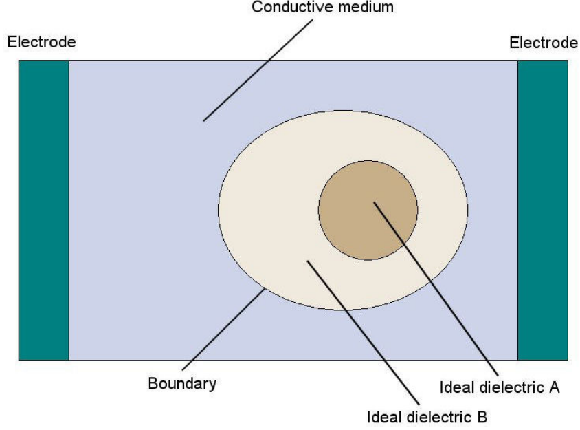
Figure 7: Example of a mixed dielectric-conductive electrostatic solution.
