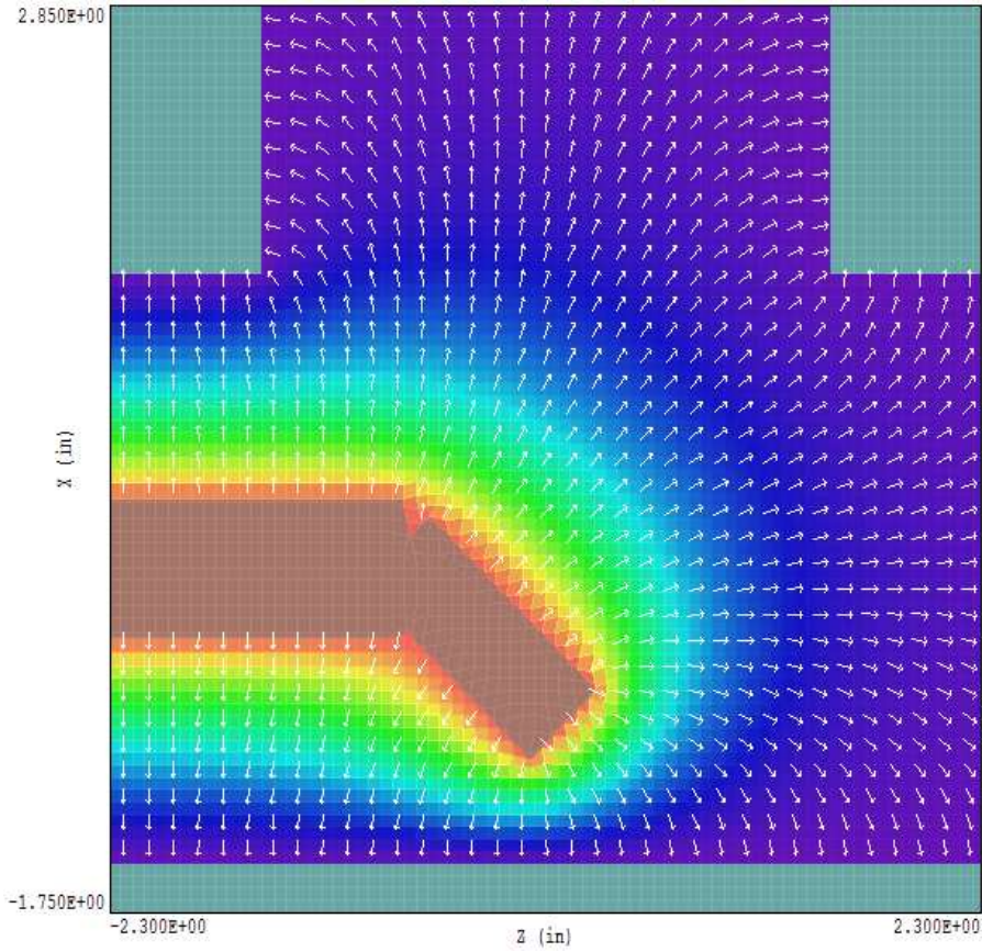
Figure 29: Element plot with electric field vectors.
