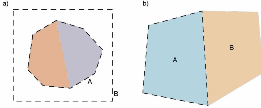
Figure 36: Surface integral of the electric stress tensor. a) Valid surfaces for an integral of electrically-active materials. A: region surfaces bounded by air elements. B: surface of an air region that encloses the electric materials. b) Invalid surface for an integral. The enclosed material current is undefined on the common boundary.
