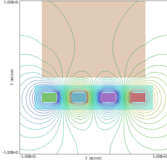
Figure 38: Calculated equipotential lines for the FORCETEST example in a plane normal to z at z = 0.0 \mu\text{m} . Dielectric: tan. Diagnostic region: cyan.
