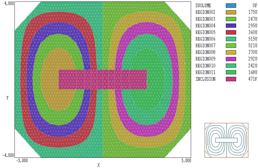
Figure 33: Mesh created with the script COSINEMEDO.MIN and the image file COSINE.DAT using the Fit option in the DataFile command and Correct = 9.
