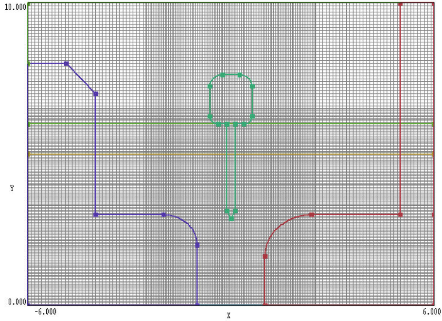
Figure 16: Modified foundation with multiple resolution zones.
