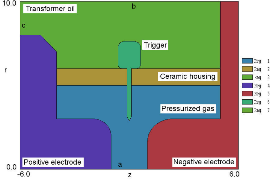
Figure 6: Application example – high-voltage spark gap switch
