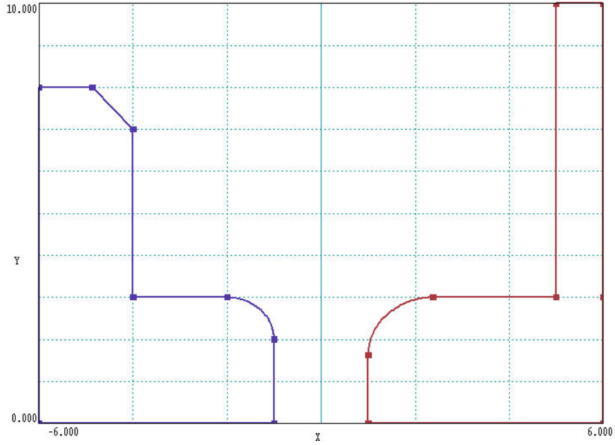
Figure 13: Completed outlines of the positive and negative electrodes.
