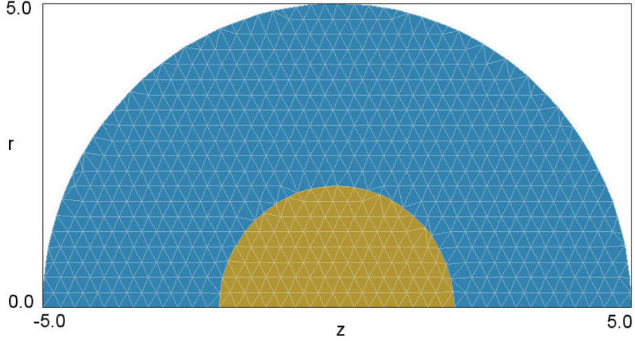
Figure 5: Spherical capacitor benchmark example with element size 0.25 cm.
