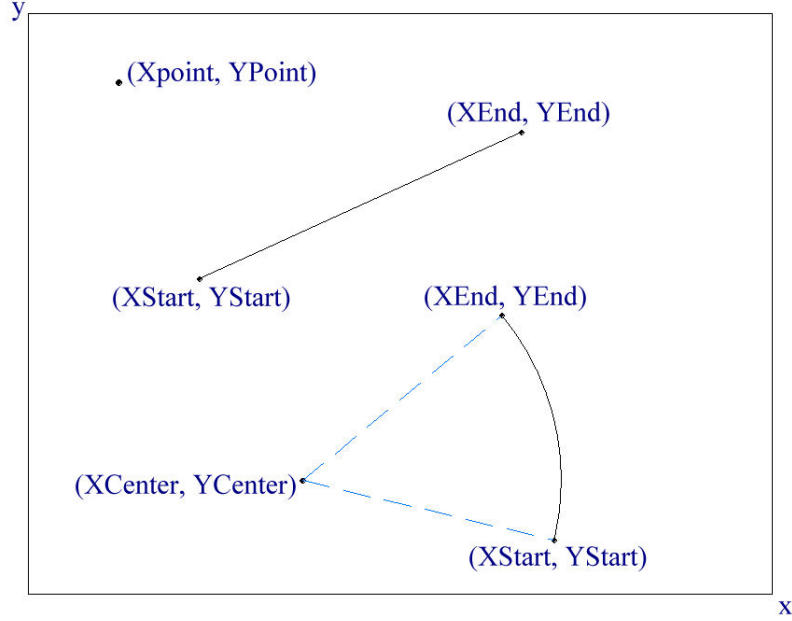
Figure 24: Parameters to define points, lines and arcs.
