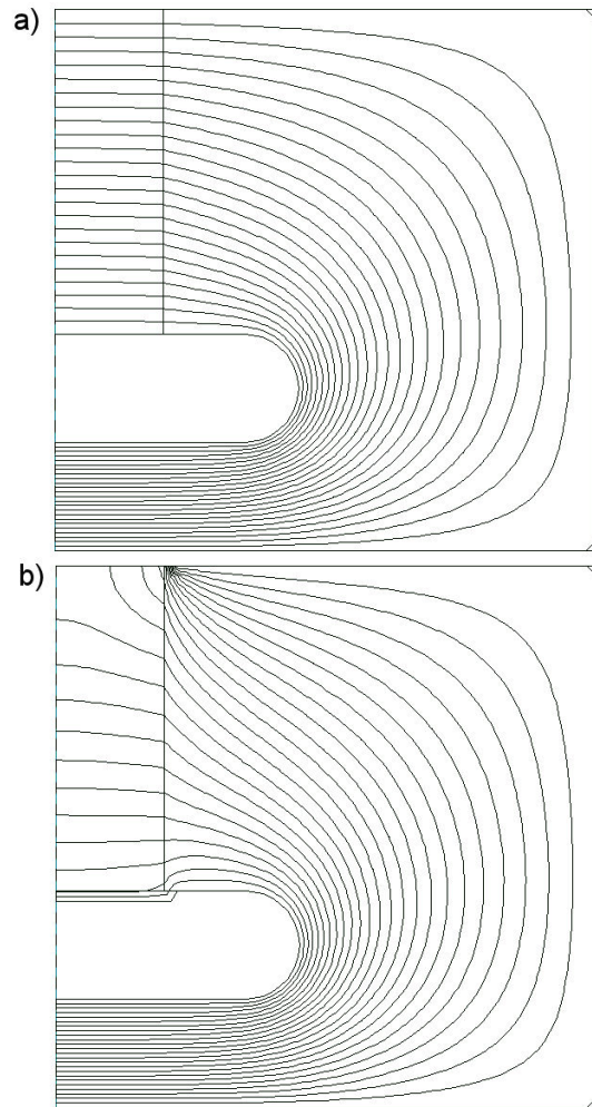
Figure 4: Equipotential lines for the example. a) Correct region ordering. b) Incorrect region ordering.
