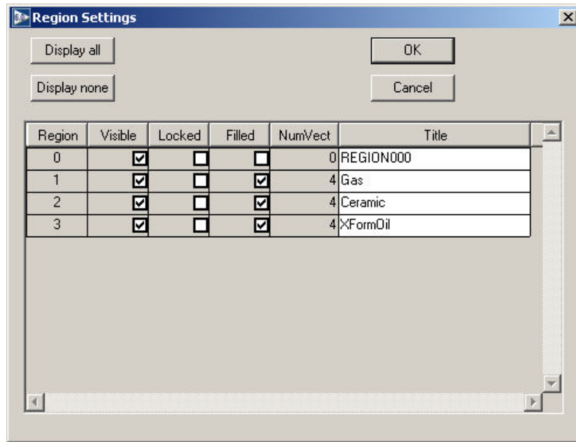
Figure 9: Dialog to set region properties.
