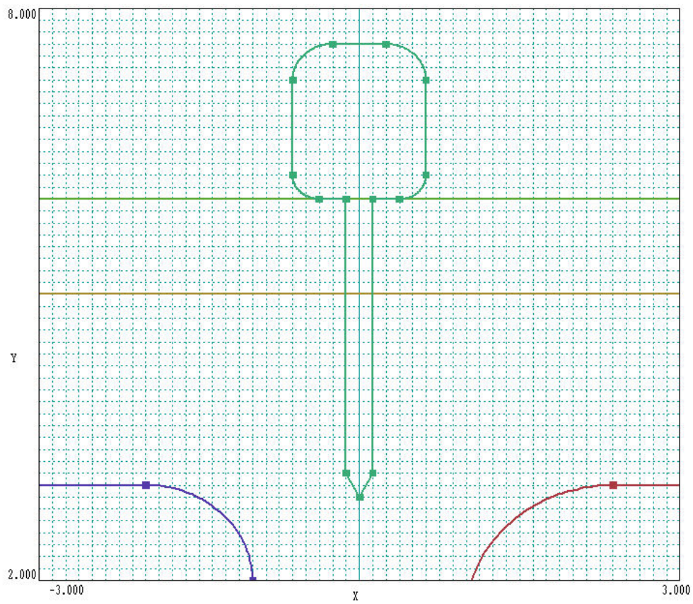
Figure 14: Drawing the trigger electrode with optimized view, snap and grid settings.
