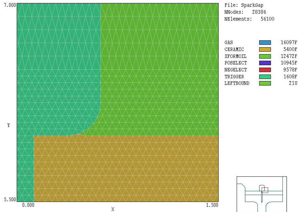
Figure 19: Plot/Repair menu – zoomed view of the SparkGap example.
