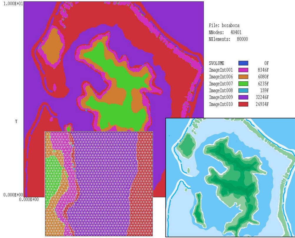
Figure 30: Generation of a conformal triangular mesh from a bitmap image. Lower right: input image. Lower left: detail of the mesh showing element boundaries.
