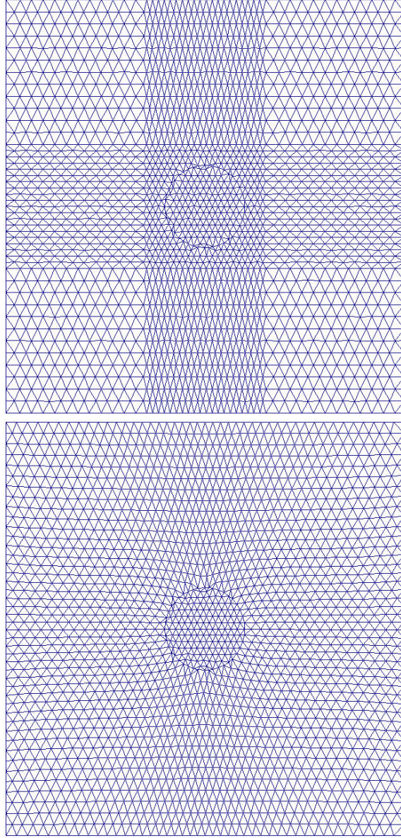
Figure 27: Variable resolution mesh without (top) and with (bottom) smoothing.
