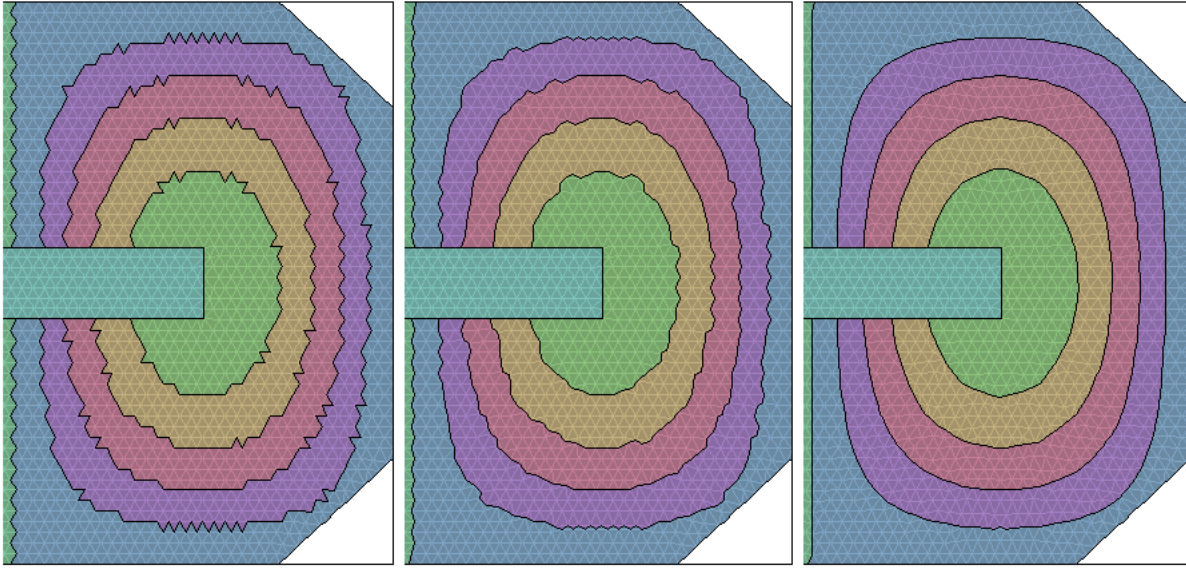
Figure 34: Section of the mesh of Fig. 33 with correction options. a) Fitting and smoothing suppressed by taking N_{Correct} = 0 . b) Smoothing for N_{Correct} = 10 cycles. c) Fitting for N_{Correct} = 10 cycles.
