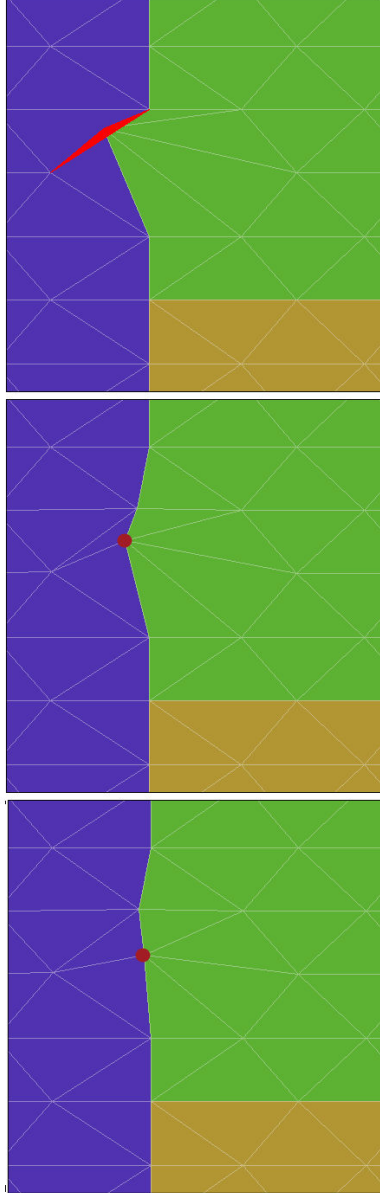
Figure 23: Element repairs. Top: inverted elements are displayed in red. Center: state of the mesh after application of the Relax bad nodes command (target node highlighted for clarity). Bottom: Further correction using the Move node command.
