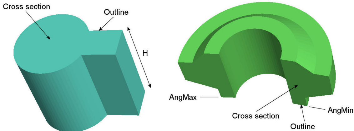
Figure 37: Fabrication parameters for extrusions (left) and turnings (right)
