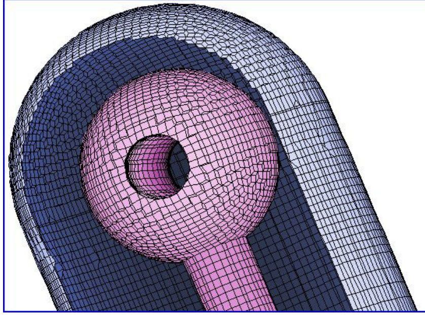
Figure 14: Cutaway view of the geometry for the simulation MESH_LOGIC.MIN . Blue facets represent the inner wall of the vacuum chamber. Violet facets show the surface of the electrode.
