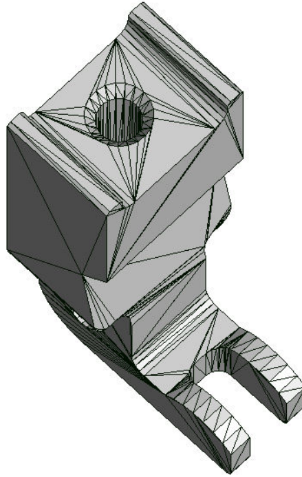
Figure 64: Typical STL object produced by a CAD program. Note that the hole and countersink require a large number of facets.
