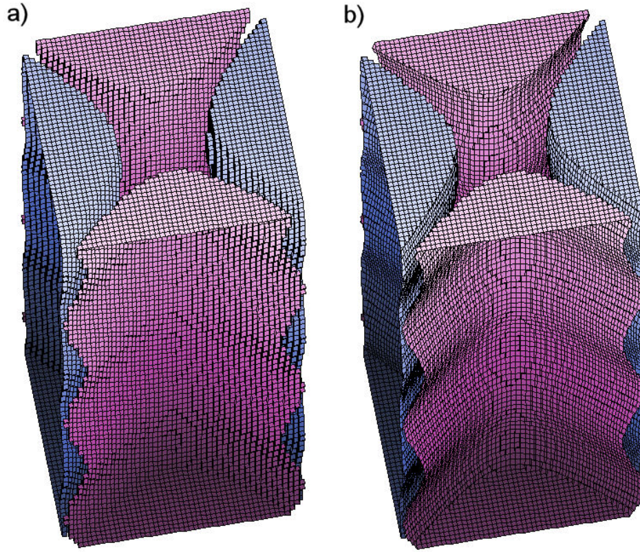
Figure 71: Electrode shapes determined from equipotential surfaces for a radio-frequency quadrupole accelerator. a) Surface fitting suppressed. b) Surface fitting applied.
