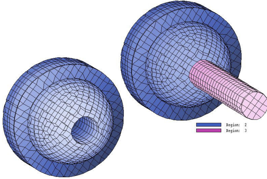
Figure 55: Example of part processing order. The rod (violet) has a higher value of PartNo than the insulator (blue). Processing of the rod creates a hole through the insulator.
