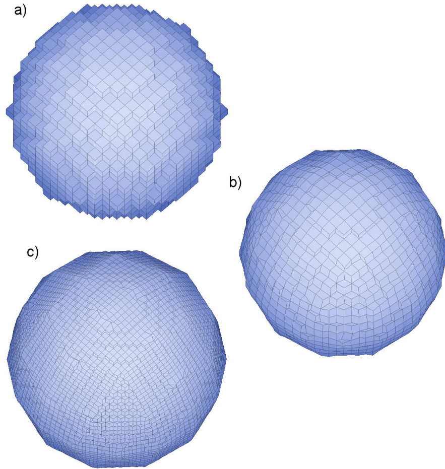
Figure 73: Hexahedron meshes created from a tetrahedron mesh of a sphere of radius 0.5 at coarse resolution. a) Hexahedron element size 0.05 with no surface fitting. b) Element size 0.05 with surface fitting. c) Element size 0.025 with surface fitting
