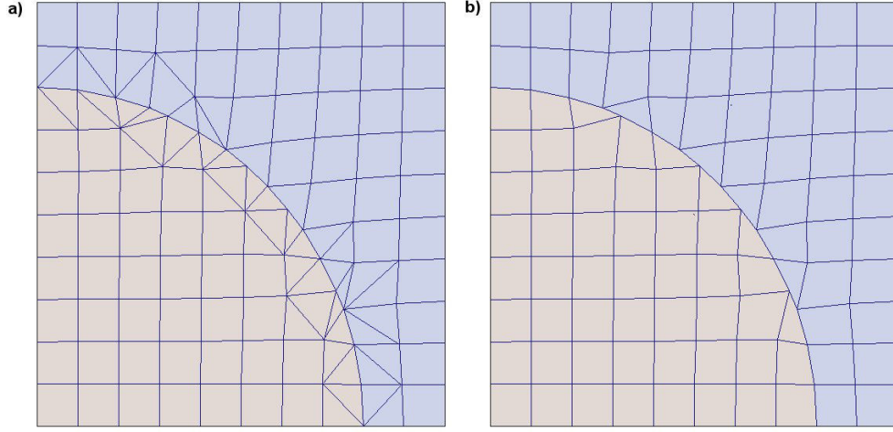
Figure 8: Two-dimensional representation of a curved surface with (a) an unstructured mesh and (b) a structured mesh.
