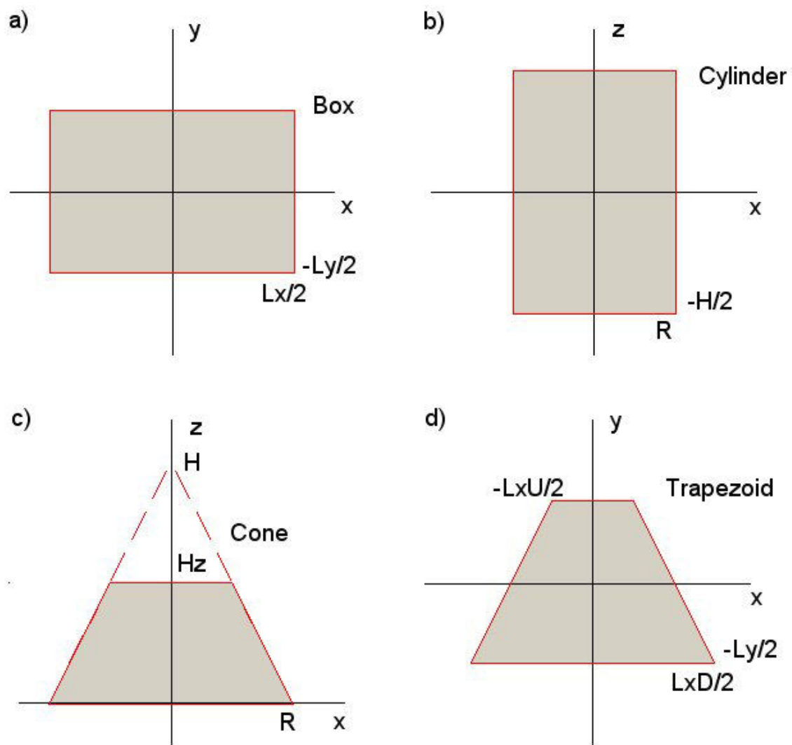
Figure 35: Basic solid shapes in the workbench frame
