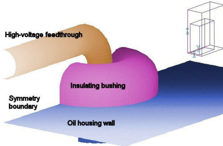
Figure 2: Geometry of the walkthrough solution
