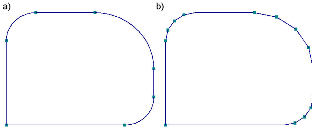
Figure 48: Effect of the Convert arcs to lines command with 22.5^\circ resolution. a) Original outline. b) After command applied.
