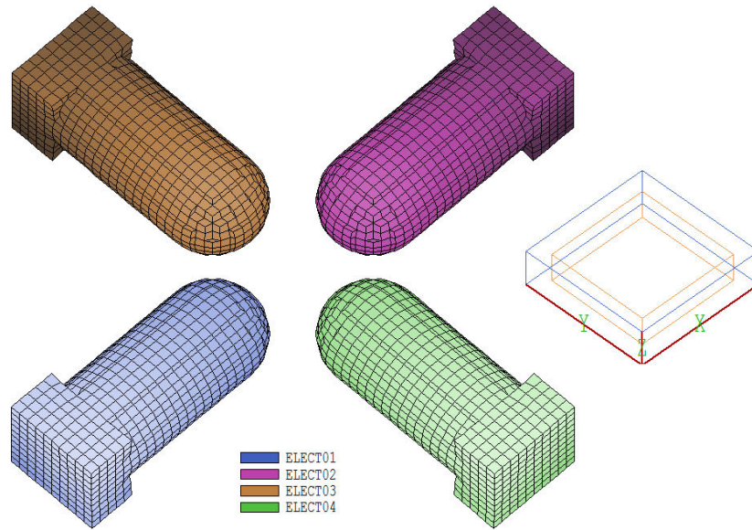
Figure 62: Macro-assembly created by rotating and positioning four assemblies using block operations.
