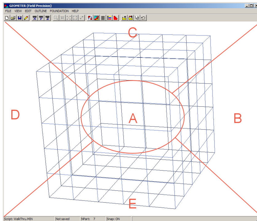
Figure 22: Perspective view of the first part (a box that fills the solution) volume showing the active zones for mouse control.
