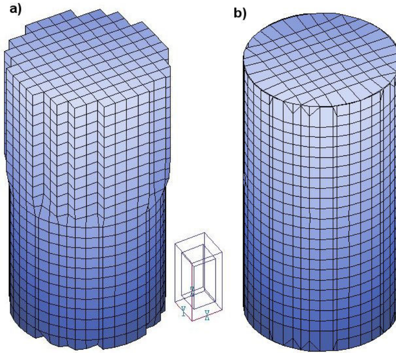
Figure 59: Fitting operations on a cylinder. a) The bottom half of the cylinder is surrounded by elements with RegNo = 1 and the top half by elements with RegNo = 2 . Only the surface bounding RegNo = 1 has been fitted. b) Appearance of the cylinder with both surface and edge fitting.
