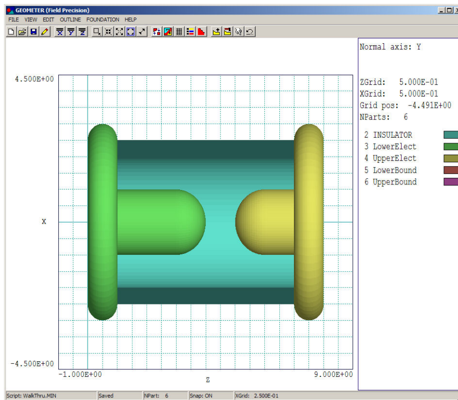
Figure 24: Assembly with insulator, upper electrode and lower electrode with the insulator displayed in a cutaway view.
