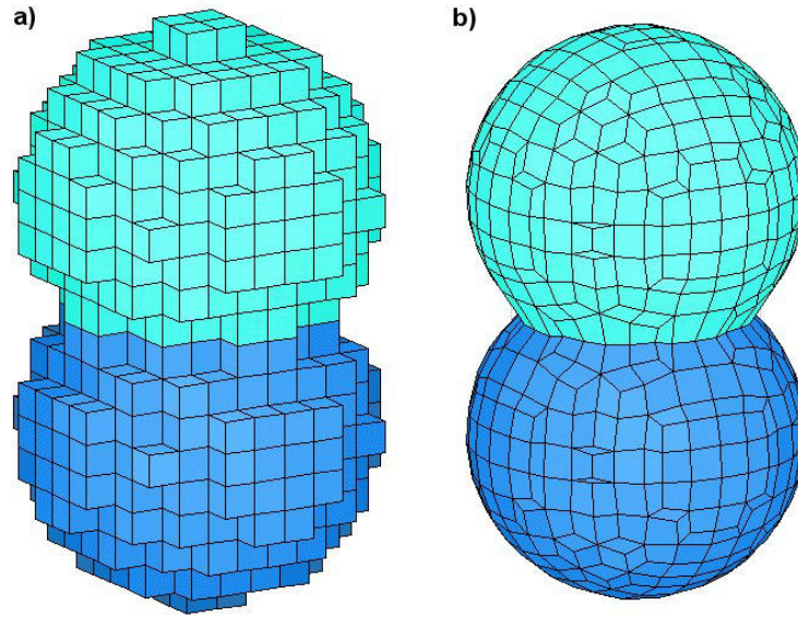
Figure 7: Representation of adjoining spheres with a) a regular mesh and b) a conformal mesh.
