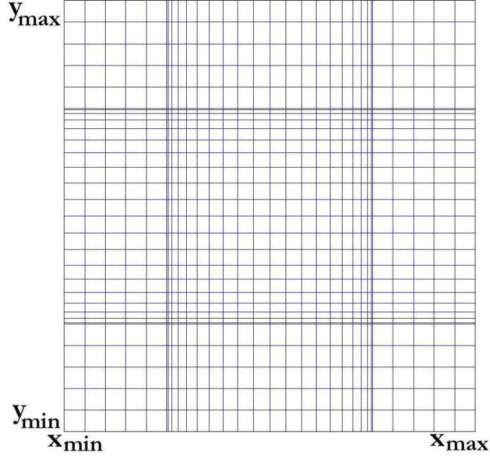
Figure 12: Foundation mesh projected in the z plane
