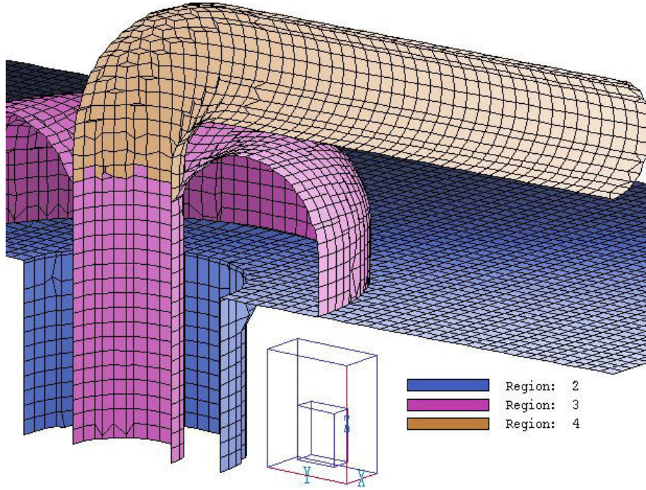
Figure 4: 3D view of region surfaces in the completed mesh
