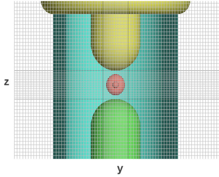
Figure 27: Detail of foundation mesh with zones of small elements defined along y and z for good resolution of the trigger electrode.
