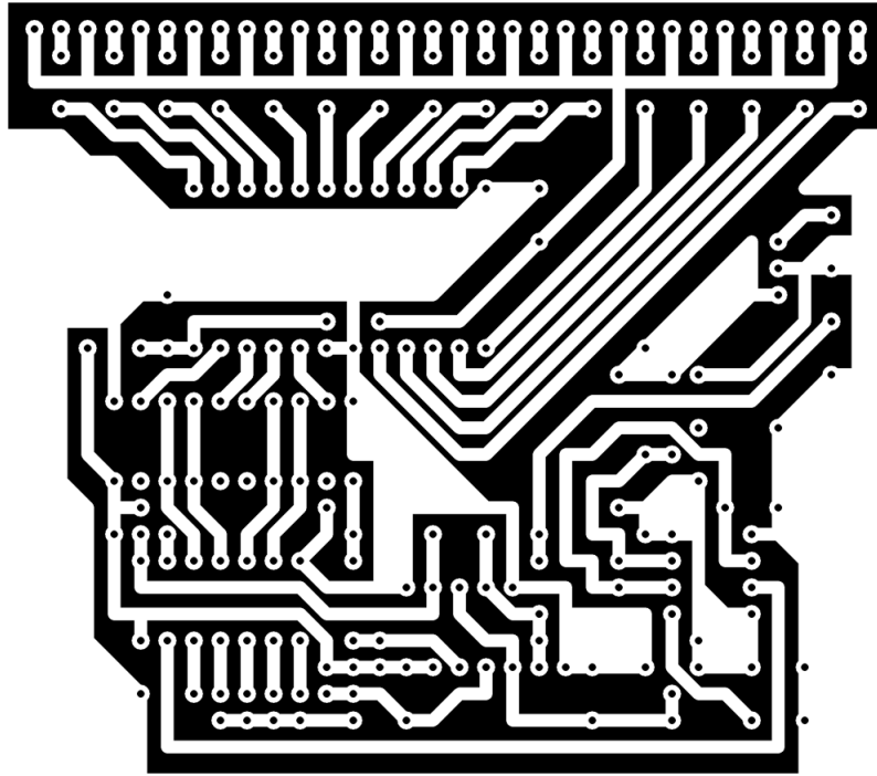
Figure 87: Printed circuit layout – conductors in white. File PC01.BMP.
