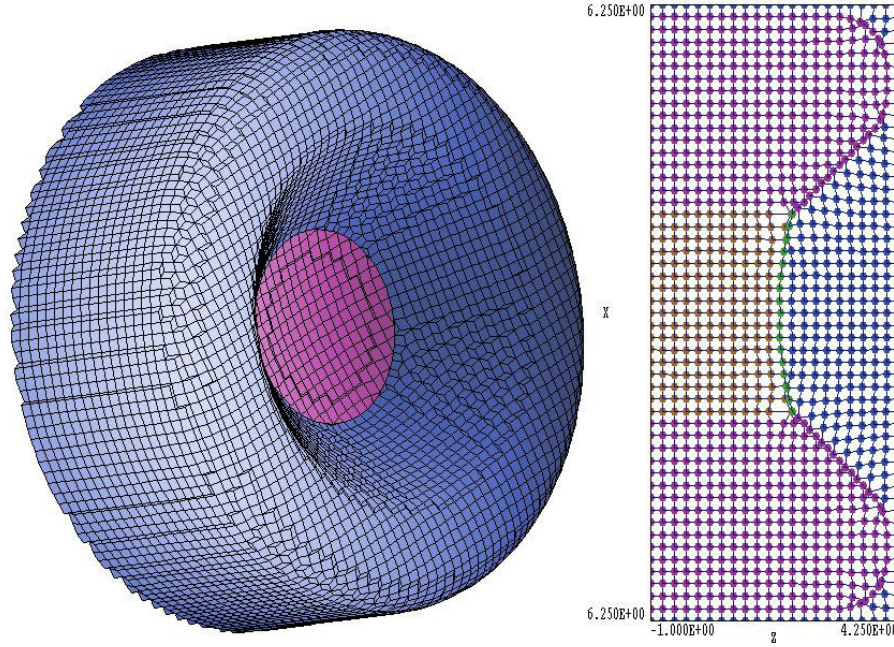
Figure 60: Example of coating operation – high-current cathode assembly. Three-dimensional view and slice through the mid-plane showing node identities. Note the coated region of nodes marked green.
