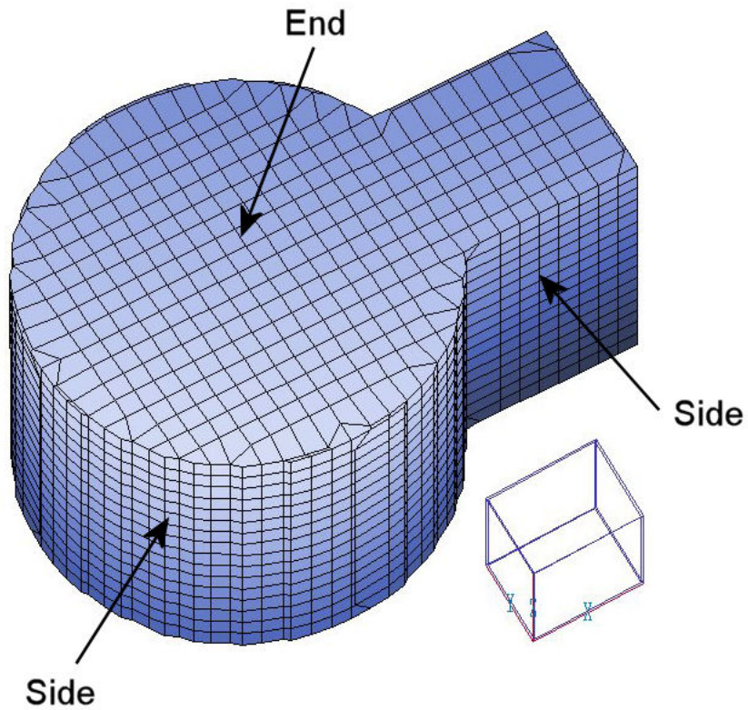
Figure 65: Extrusion with selective surface and edge fitting.
