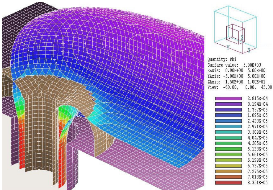
Figure 6: Electrostatic solution using the HiPhi program. Surface of \phi = 5 kV color-coded by |\mathbf{E}| .
