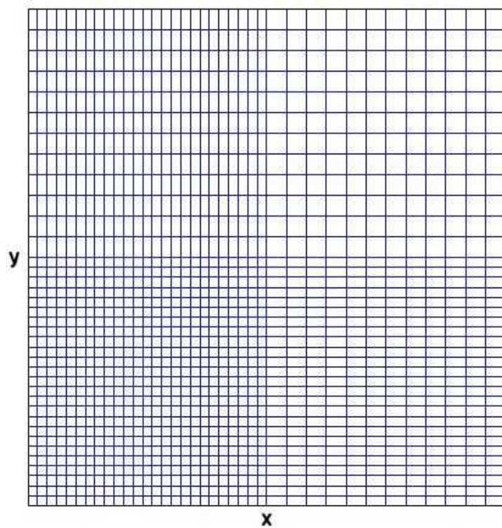
Figure 53: Variable-resolution mesh.
