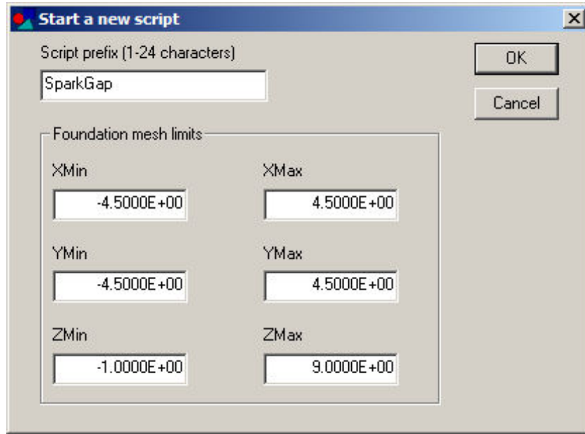
Figure 18: Dialog to begin a new script
