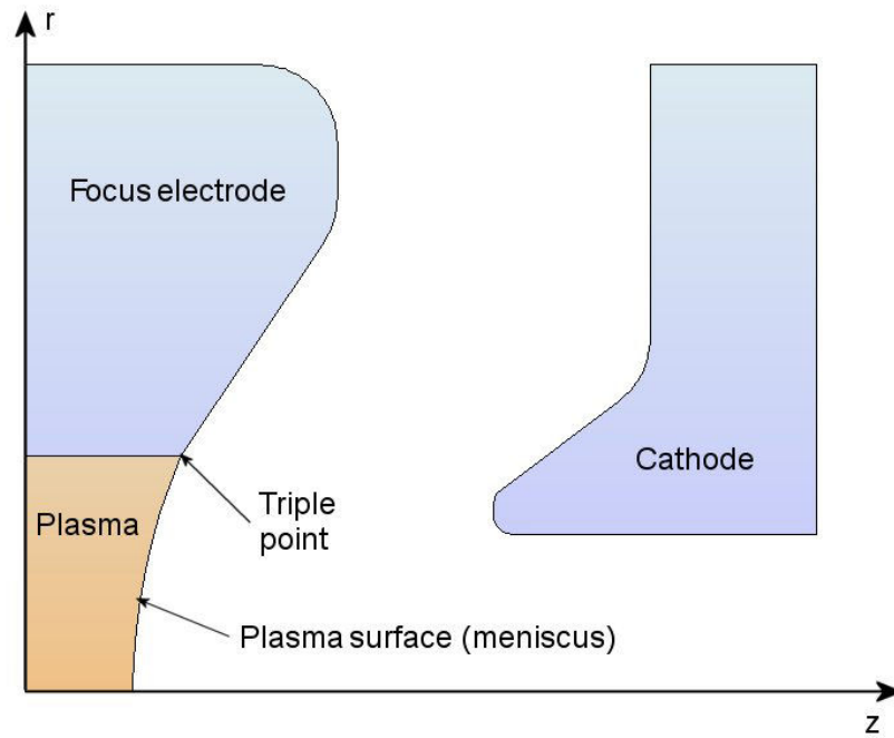
Figure 29: Terminology for ion extraction from a free plasma surface.
