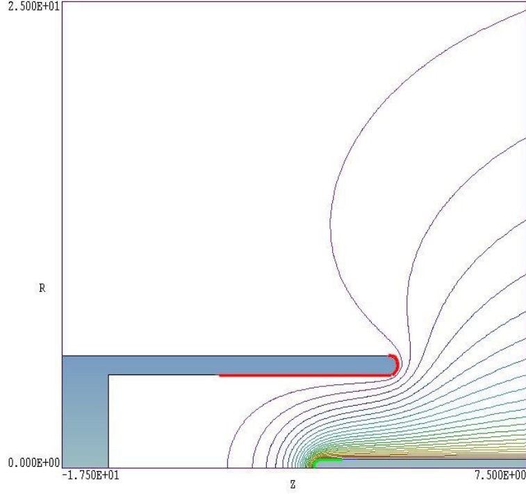
Figure 27: Geometry of the PINCHBEAM example – magnified view of the acceleration gap. Red line: electron emission region on the cathode. Green line: ion emission region on the anode.
