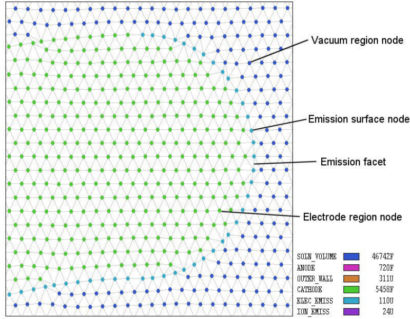
Figure 19: Definition of an emission surface on a conformal triangular mesh.
