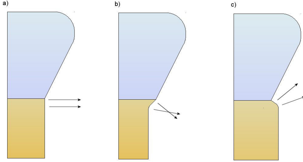
Figure 31: Balancing plasma flux j_p with space-charge-limited flux j_C to achieve a smooth connection at the triple point. a) Ideal balance. b) Insufficient plasma flux. c) Excess plasma flux.
