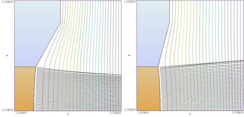
Figure 35: Self-consistent plasma surface shape, equipotential lines and model particle trajectories. Left: example PLASMA02 with \theta = 30.0^\circ . Right: example PLASMA03 with \theta = 15.0^\circ .
