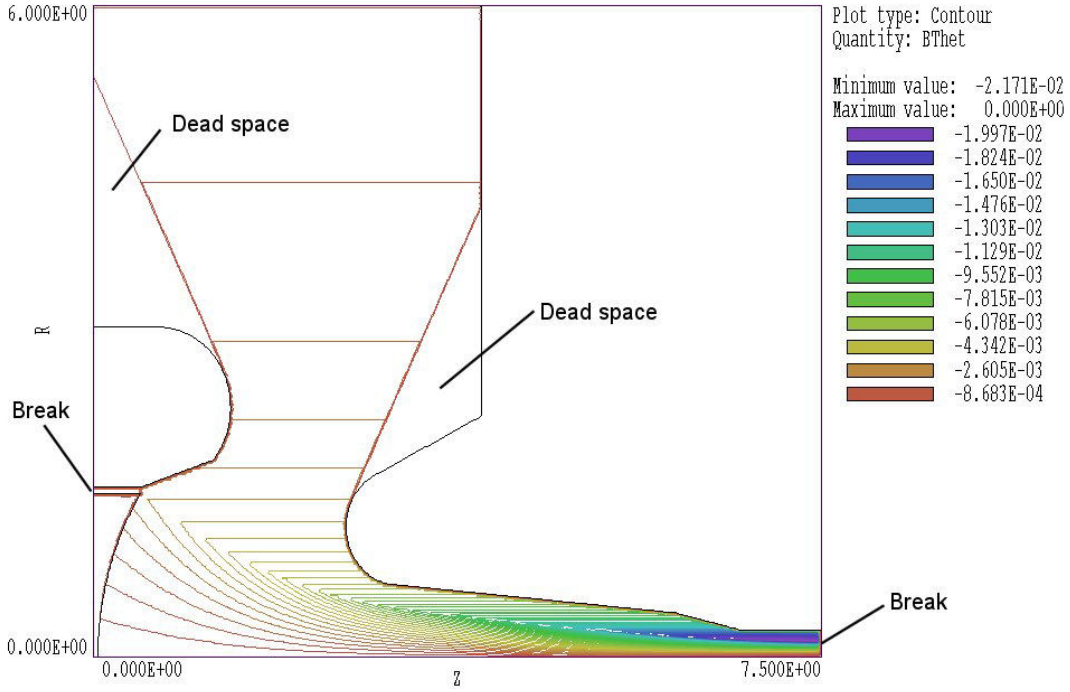
Figure 25: Contour lines of B_\theta showing missing values in areas shaded by re-entrant collector surfaces that do not connect to the axis.
