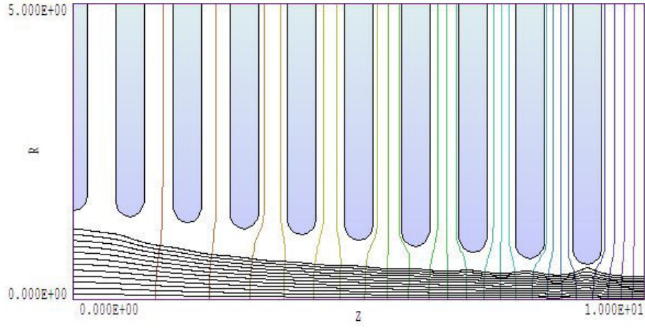
Figure 22: Ion-mobility spectrometer – electrode geometry and ion trajectories.
