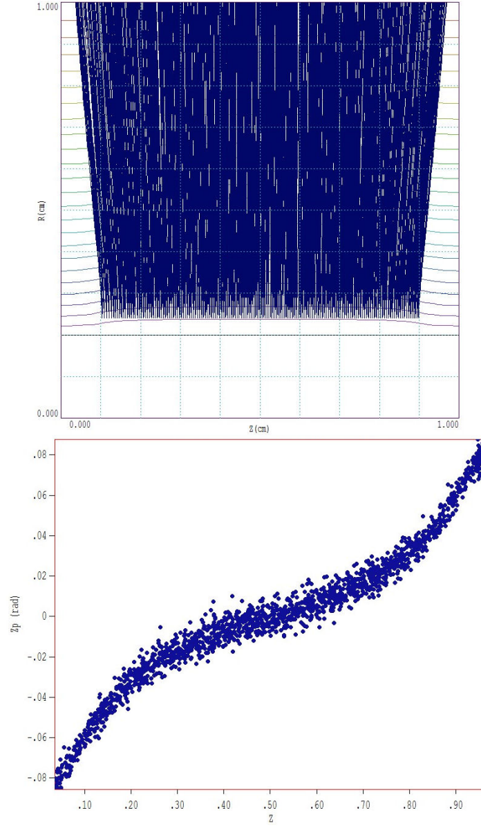
Figure 23: Particles generated at an emission surface with source temperature. Outward radial flow of electrons across a 5000 V gap with kT_s = 0.25 eV. Top: equipotential lines and particle trajectories. Bottom: axial phase space plot at the outer boundary. The predicted angular divergence is \Delta\theta \cong \sqrt{kT_s/5000} = 0.007 .
