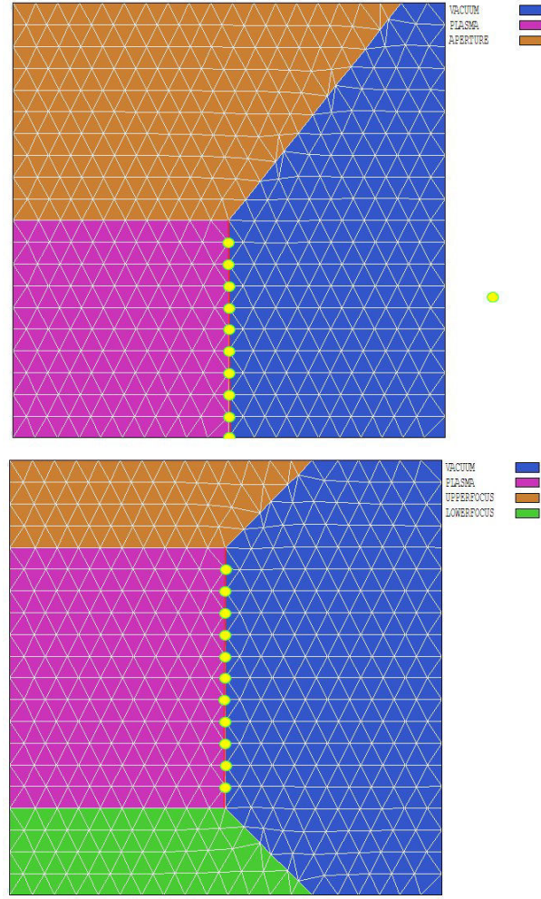
Figure 32: Definition of plasma facets (red line) and plasma nodes (yellow dots). Plasma elements are colored violet and vacuum elements are colored blue. Top: Disk plasma with symmetry axis on the lower edge. Bottom: Annular plasma.
