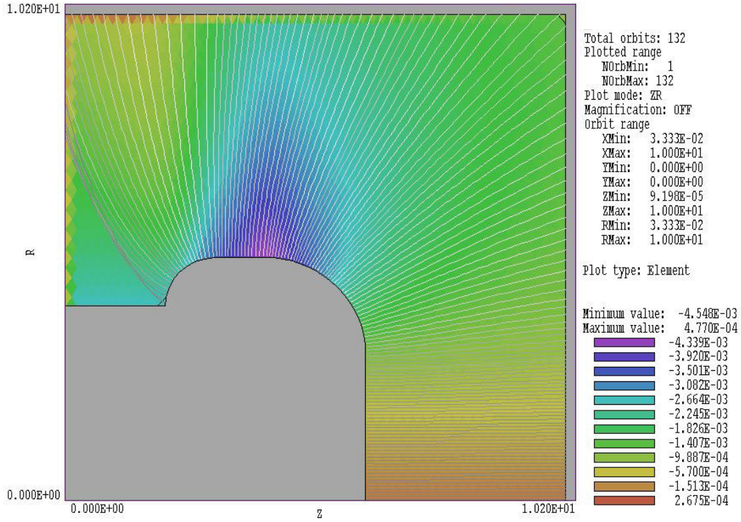
Figure 26: Variations of B_\theta for electron emission from a convex cathode.
