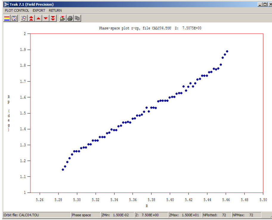
Figure 18: Distribution plot menu showing a phase space plot for an annular beam.
