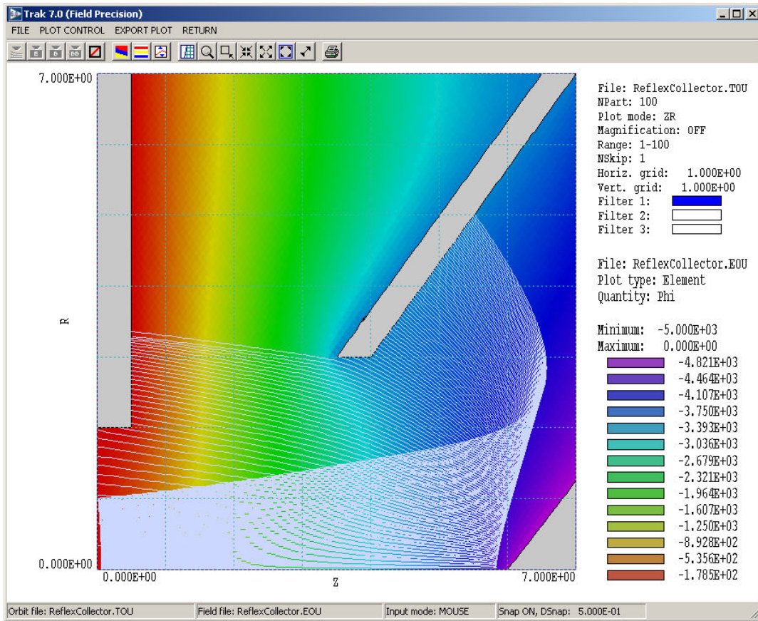
Figure 14: Working environment for creating trajectory/field plots.
