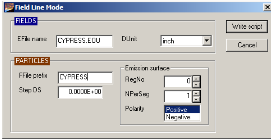
Figure 8: Run setup dialog – FLine mode.
