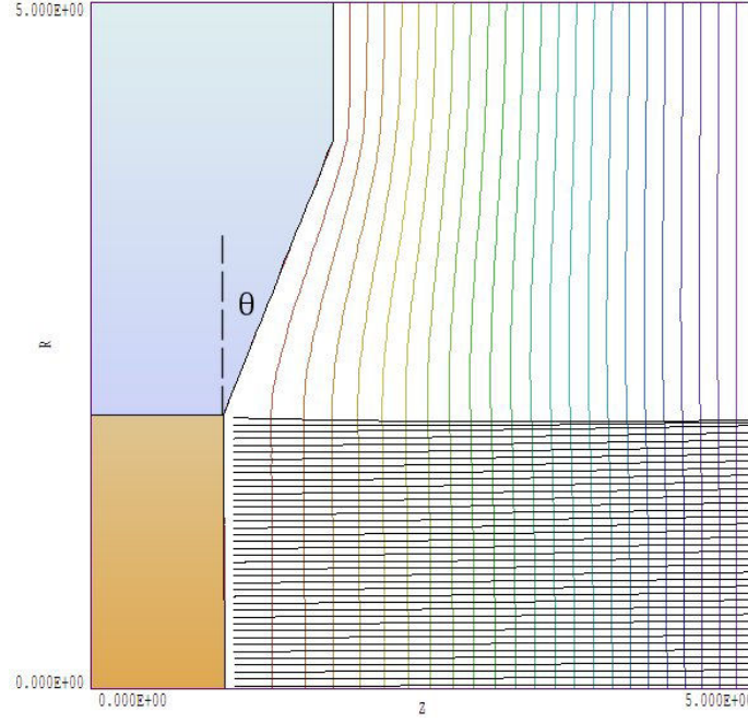
Figure 33: Geometry of the example PLASMA01 with focusing electrode angle \theta = 22.5^\circ . Figure shows the self-consistent plasma surface, equipotential contours and model particle trajectories. Dimensions in cm.
