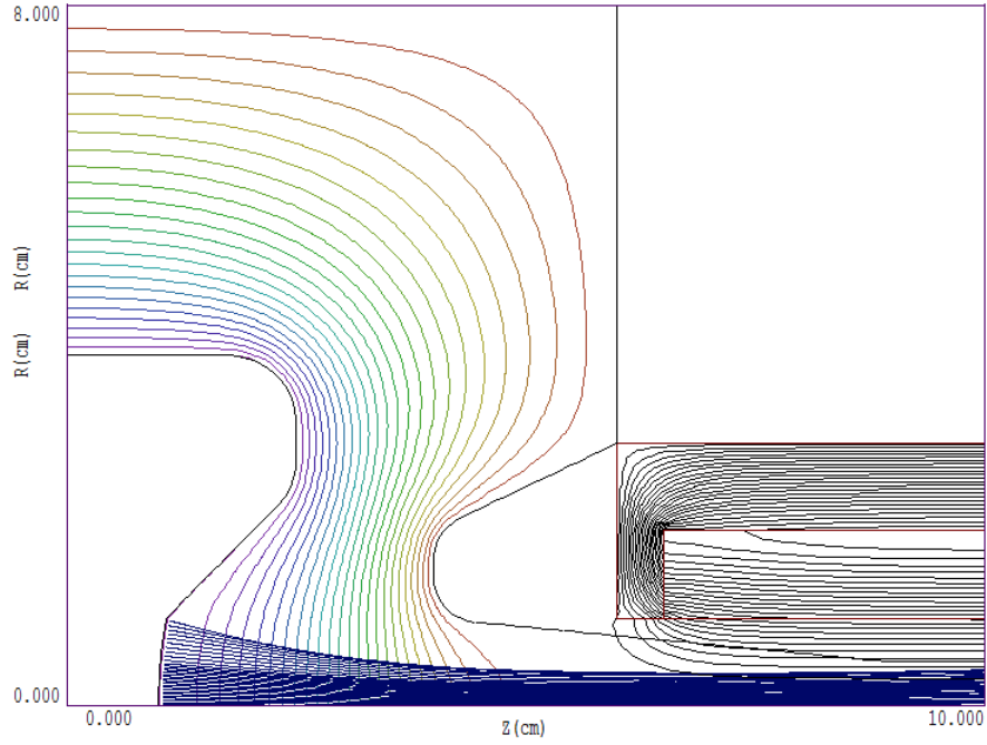
Figure 17: Plot combining particle trajectories, electrostatic equipotential lines, magnetic field lines and region boundaries in both field solutions.
