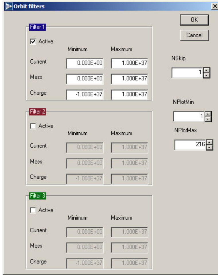
Figure 16: Dialog to set filter criteria for the display of particle trajectories.
