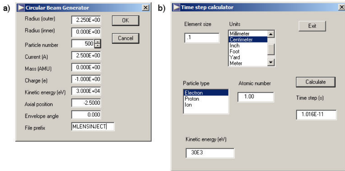
Figure 13: Utilities in the Tool menu. a) Circular-beam generator. b) Time-step calculator.
