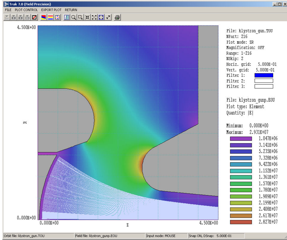
Figure 1: Screenshot – Trak in the trajectory plotting mode.
