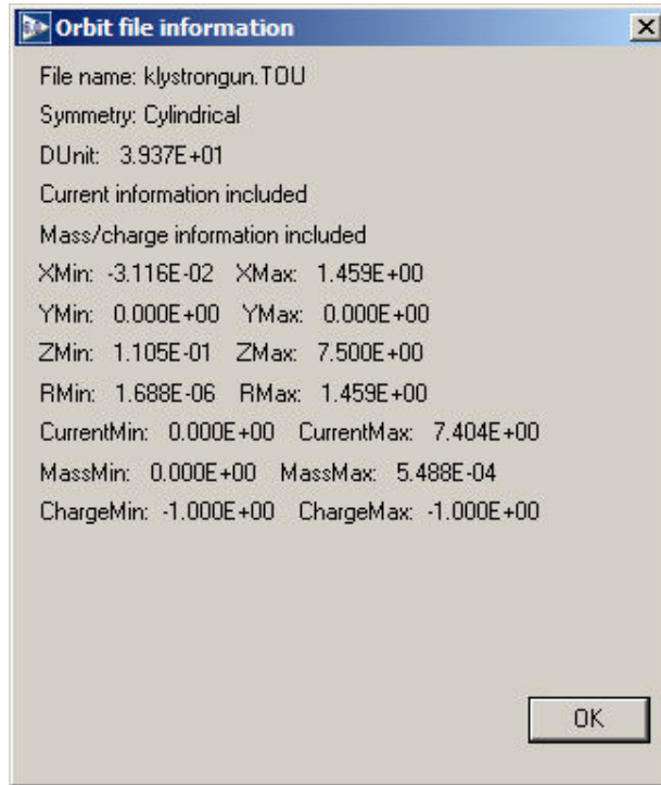
Figure 15: Information on the currently-loaded trajectory file displayed in a message box.
