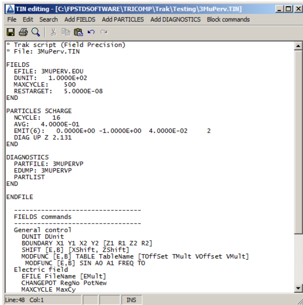
Figure 12: Screen display of the Trak input file editor.
