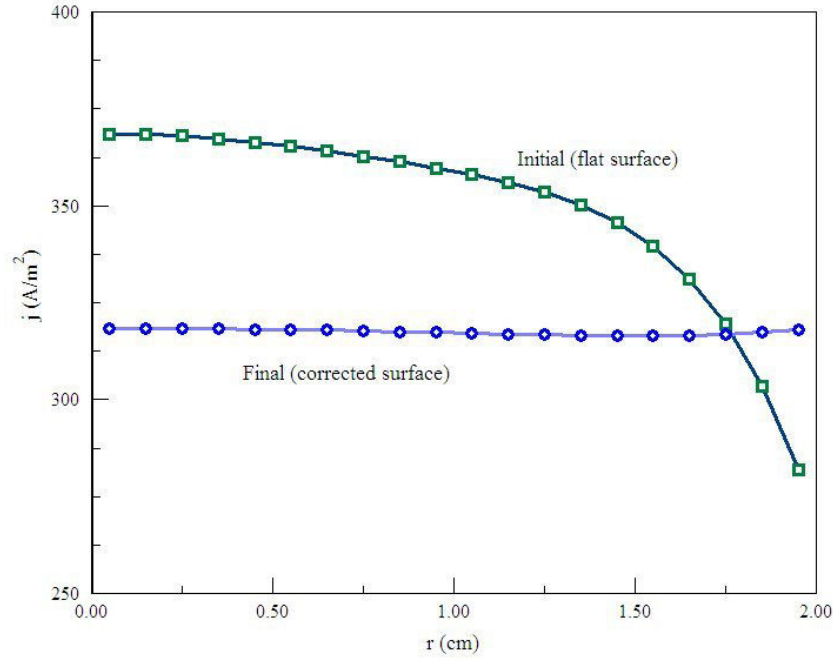
Figure 34: Radial variation of current density for example PLASMA02 with \theta = 30.0^\circ . Green curve shows the initial state while the blue curve shows the current density after the iterative plasma surface adjustment.
