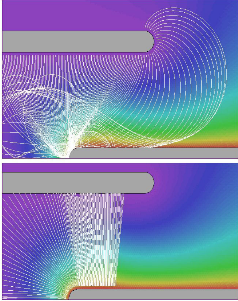
Figure 28: Electron (top) and ion trajectories (bottom) for the PINCHBEAM example with NSkip = 5 . Color-coding follows the electrostatic potential.
