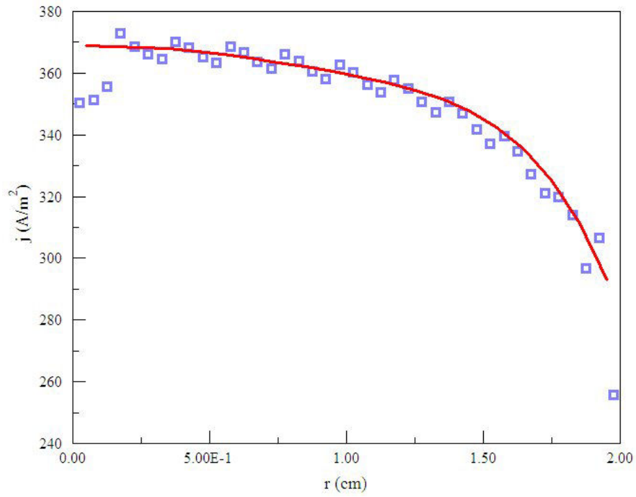
Figure 36: Weighted current-density smoothing for a cylindrical beam. Blue squares represent values for individual model particles, the red line is a fourth-order fit. Note the effects of small interpolation errors at element boundaries and near the axis.
