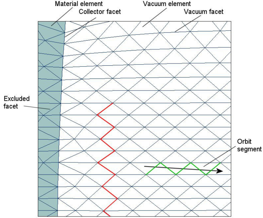
Figure 24: Definition of terms for the calculation of beam-generated magnetic field on a conformal mesh. Red lines show the path from a node to the axis along facets. Green lines show facets intersected by a trajectory segment.
