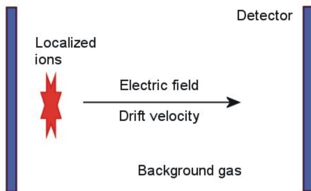
Figure 21: Principle of the ion-mobility time-of-flight spectrometer.
