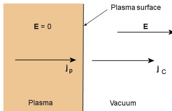
Figure 30: One-dimensional extraction from a free plasma surface.
