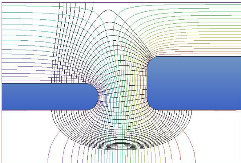
Figure 20: Field lines generated from an emission surface on the left electrode.
