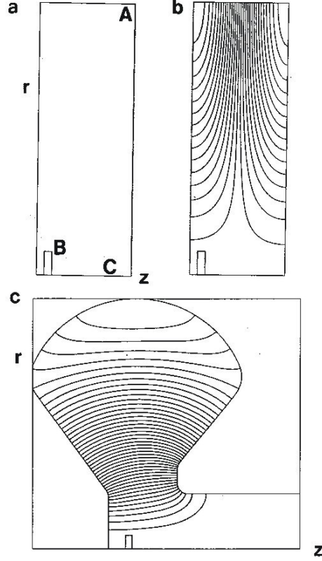
Figure 40: Resonant modes in cylindrical cavities. a) Pillbox geometry. For H type solutions metal walls are open circuit boundaries and rH_\theta = 0 on axis. Location of drive current and sensing probe shown. Cavity radius: 0.70 m. Cavity length: 0.25 m. b) Contours of rH_\theta (electric field lines) for the TM_{011} mode at 621.329 MHz. c) Contours of rH_\theta for the TM_{010} mode in a klystron cavity.
