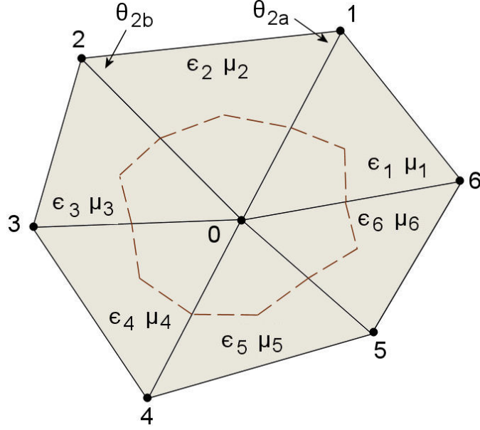
Figure 32: Relative numbering of nodes and elements in the structured, conformal triangular mesh. The dashed line passes through the midpoints of facets and the centers-of-mass of elements.
