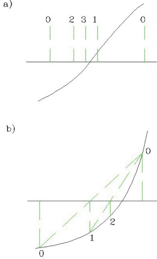
Figure 39: Numerical determination of zero crossing point of a function. a) Bisection method. b) False position method.
