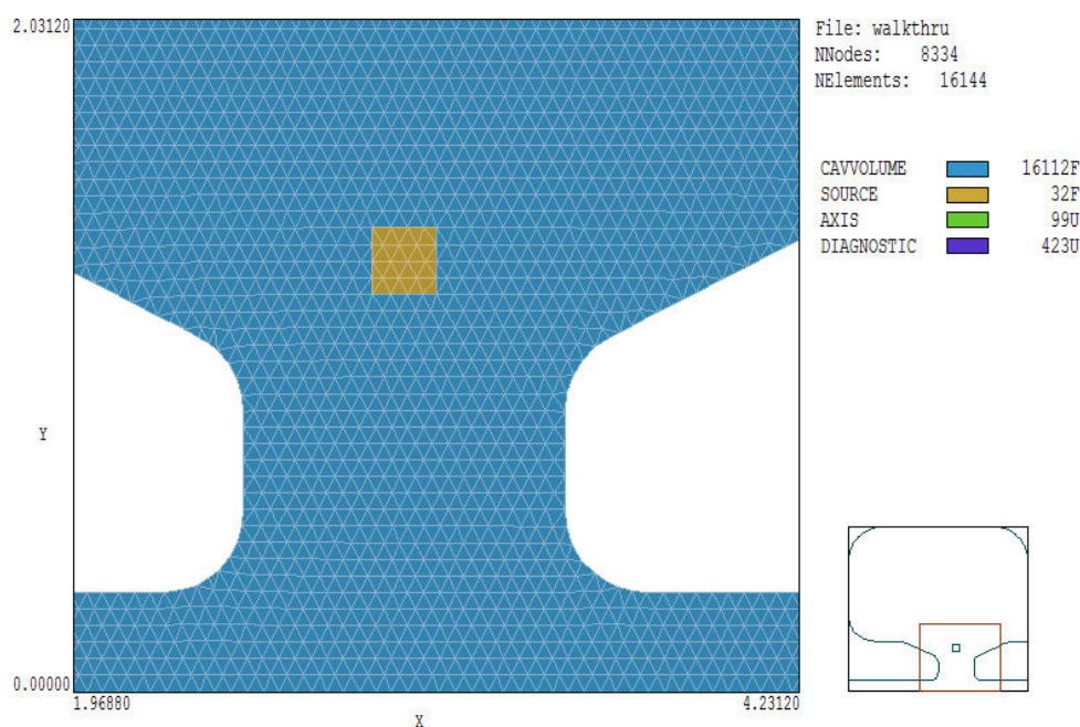
Figure 5: WALKTHRU example – detail of completed mesh.
