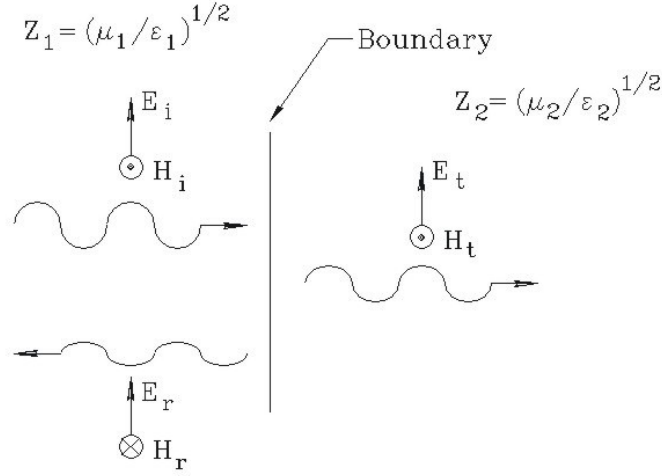
Figure 31: Traveling wave incident on a boundary between media with different impedances.
