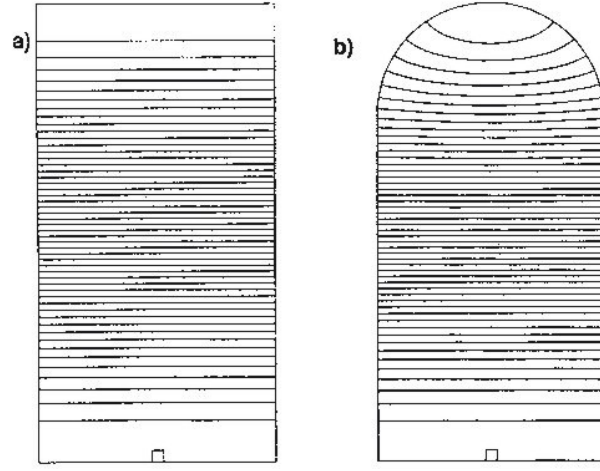
Figure 43: Comparison of the Q factors for two 303 MHz accelerators cavities with the same axial length cavities. Contours of rH_\theta , lower boundary is the z axis. a ) Pillbox cavity, outer radius 0.3789 m. b ) Cavity with contoured outer wall, outer radius 0.4000 m.
