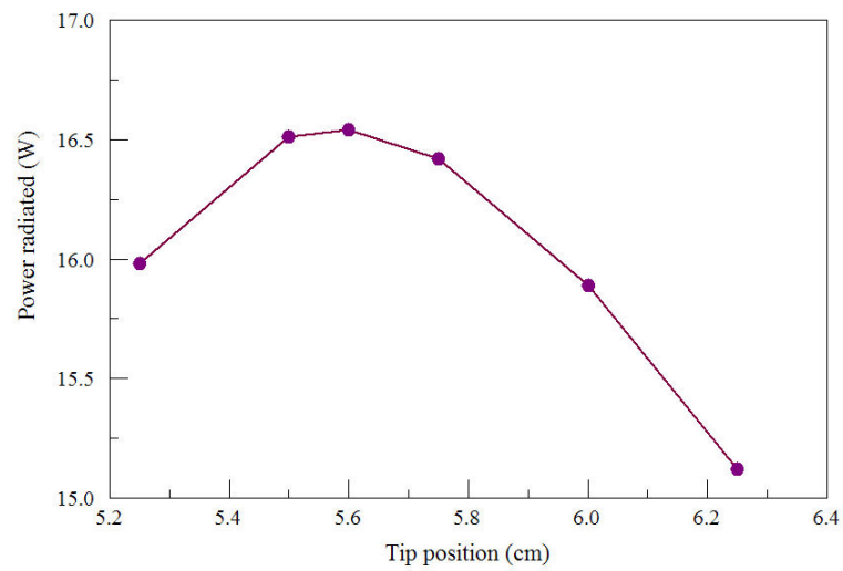
Figure 27: Example QUATWAVE, radiated power as a function of the antenna length
