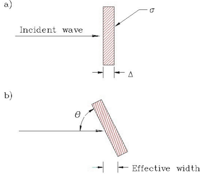
Figure 34: Absorbing boundary for two-dimensional solutions. a) Normal incidence, \theta = 90^\circ . b) Increase in effective layer thickness for \theta < 90^\circ .
