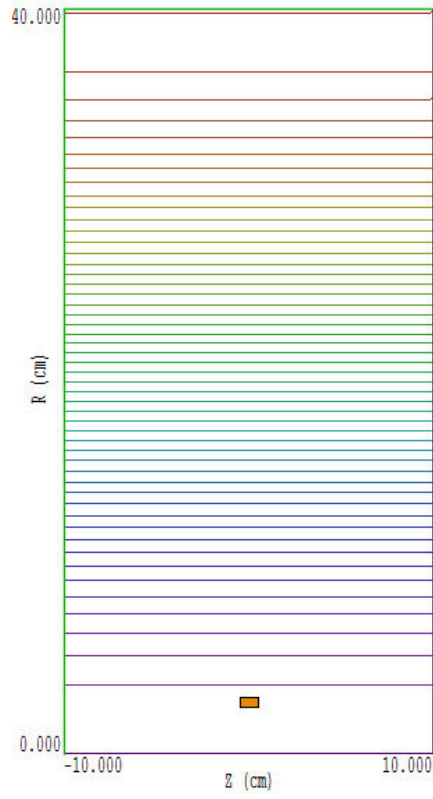
Figure 15: Geometry for the SimpleCavity example with electric field lines. The drive current region is shown in orange and the diagnostic boundary in green.
