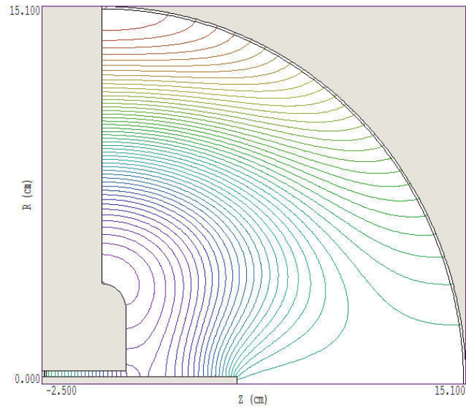
Figure 26: Example QUATWAVE, electric field lines
