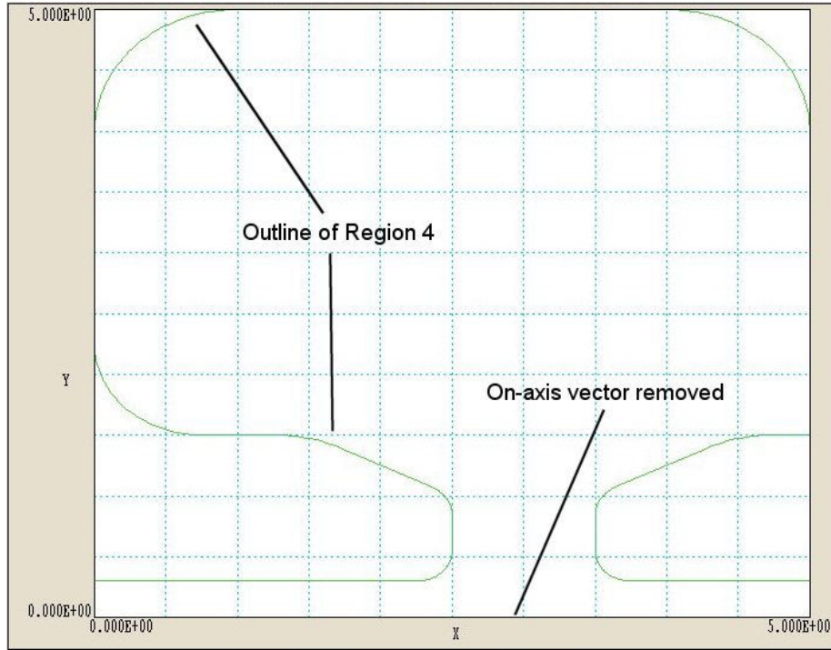
Figure 4: WALKTHRU example – Region 4 with on-axis vector removed.
