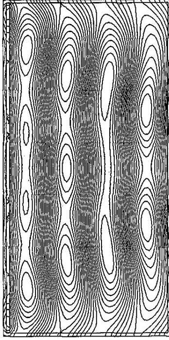
Figure 44: Unsuccessful approach to generate plane waves in an anechoic chamber. Vacuum region surrounded by matched termination layer with a planar drive current layer at the left. The plot shows lines of \mathbf{H} – waves travel from left to right.
