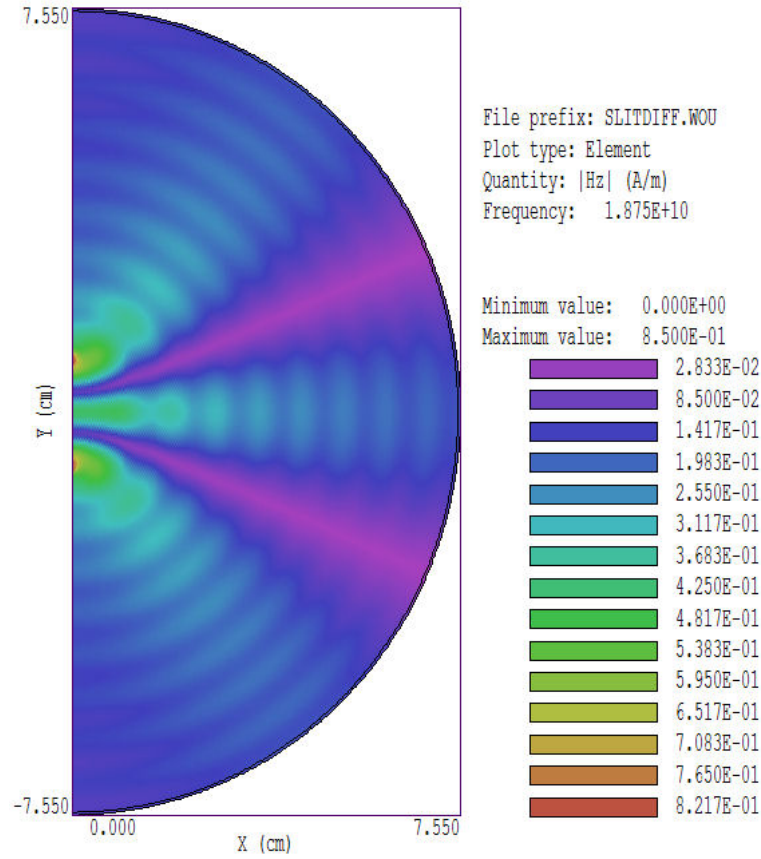
Figure 22: Example SLITDIFF, plot of |H_z| .
