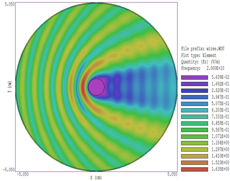
Figure 29: Example WIREE, plot of |E_z| , total fields.
