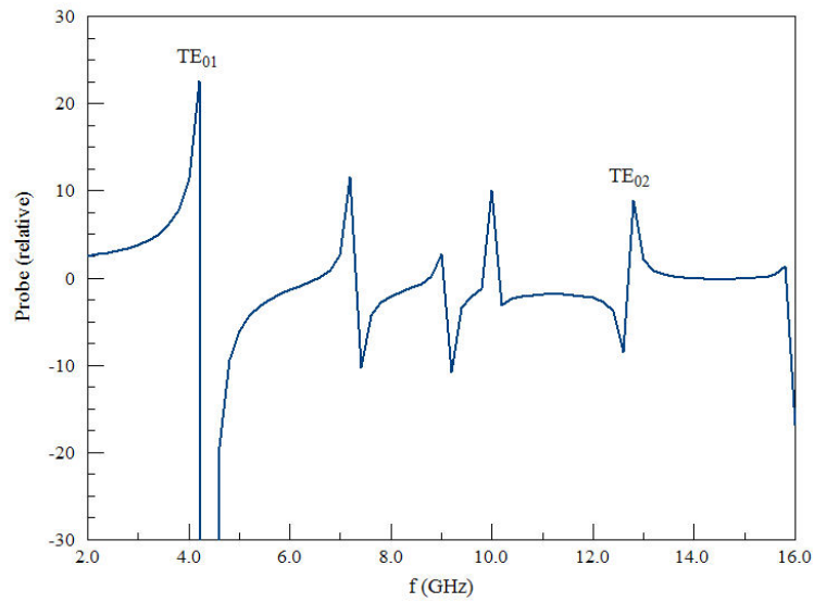
Figure 16: Frequency scan of TE cutoff modes in a circular waveguide of radius R = 2.0 cm.
