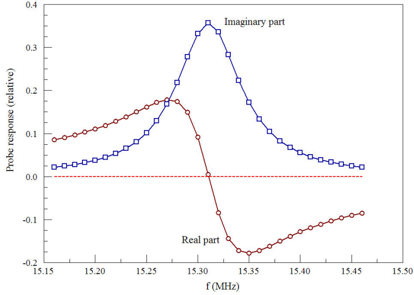
Figure 20: Probe response versus frequency for the SYNCHCAV example.
