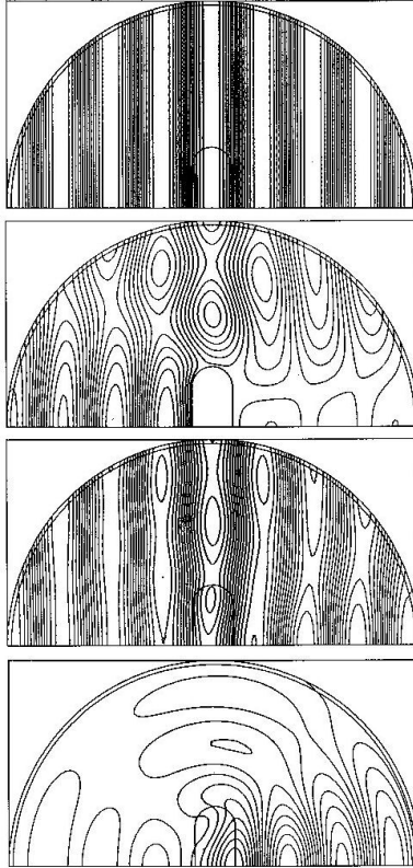
Figure 45: Scattering solutions using the distributed source method. a) Ideal plane E waves created by a distributed source. b) Total field in the presence of a conducting body ( \epsilon = 10^5\epsilon_0 ). c) Total field in the presence of a dielectric body ( \epsilon = 1.5\epsilon_0 ). d) Isolated scattering fields from the dielectric body of part c .
