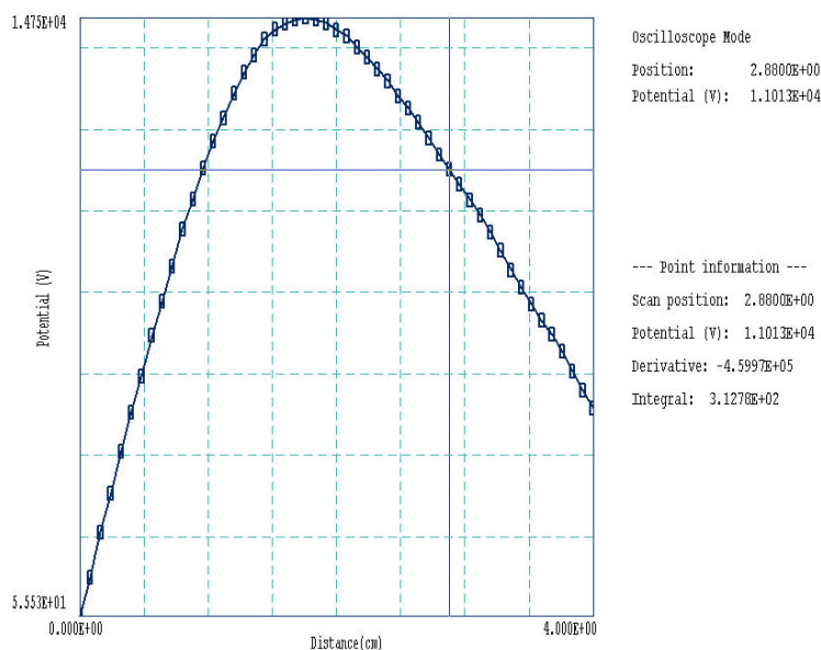
Figure 14: Scan plot in the oscilloscope mode
