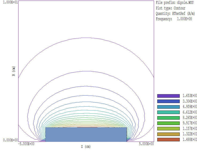
Figure 24: Contours of |H_\theta| at \phi = 0^\circ for the DIPOLE example at 100 MHz.
