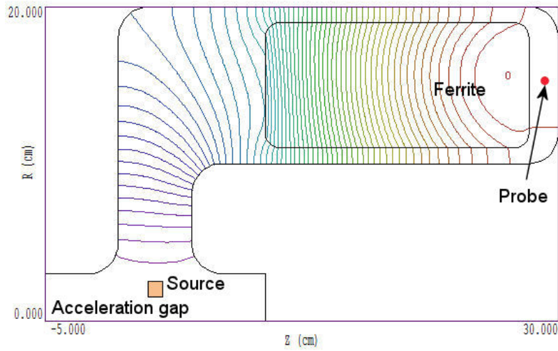
Figure 19: Geometry of the SYNCHCAV example, electric field lines at 15.31 MHz.
