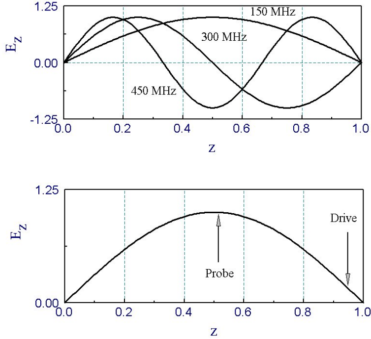
Figure 36: Lower order E wave modes of a one-dimensional vacuum resonator. For L = 1 m, the predicted resonant frequencies are f_1 = 149.8962 MHz, f_2 = 299.7925 MHz and f_3 = 449.6887 MHz.
