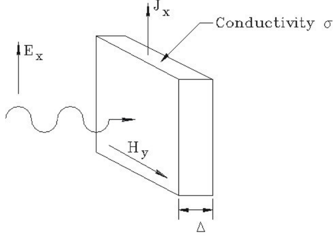
Figure 33: Traveling wave incident on a matched resistive layer.
