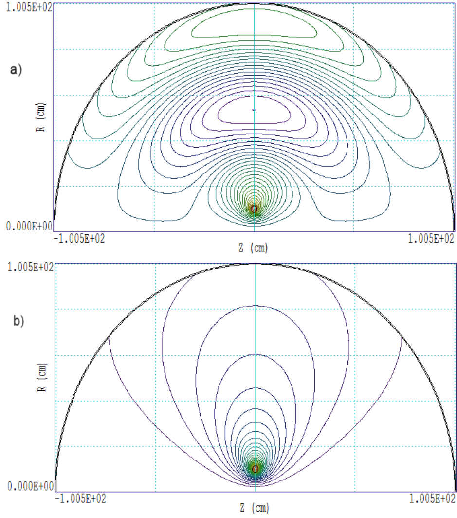
Figure 28: Magnetic dipole antenna model, lines of |\mathbf{H}| . Circular wire loop inside a spherical anechoic chamber. a) f = 400.0 \text{ MHz} . b) f = 80.0 \text{ MHz} .
