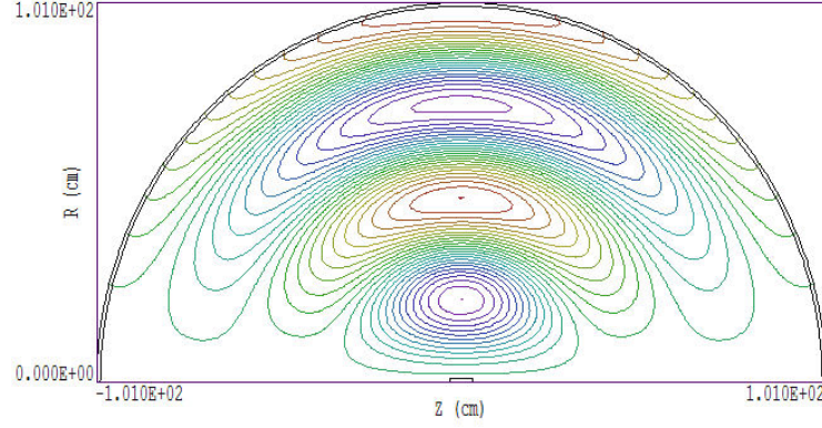
Figure 23: Electric field lines from a dipole current, f = 600 MHz, phase \phi = 90^\circ .
