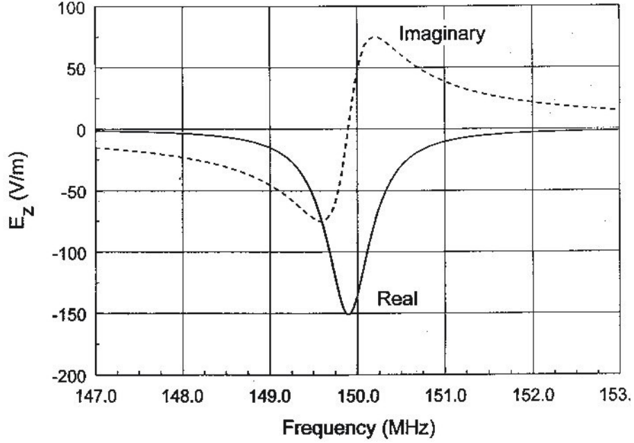
Figure 38: Resonant circuit – variation of V as a function of \Omega near resonance. Drive current I_0 = [1, 0] , Q = 250 .
