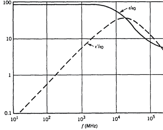
Figure 35: Real and imaginary parts of the relative dielectric constant of purified water as a function of frequency. (Adapted from J.B. Halstead, Liquid Water – Dielectric Properties in Water – a Comprehensive Treatise , F. Franks, ed., Plenum, New York, 1972).
