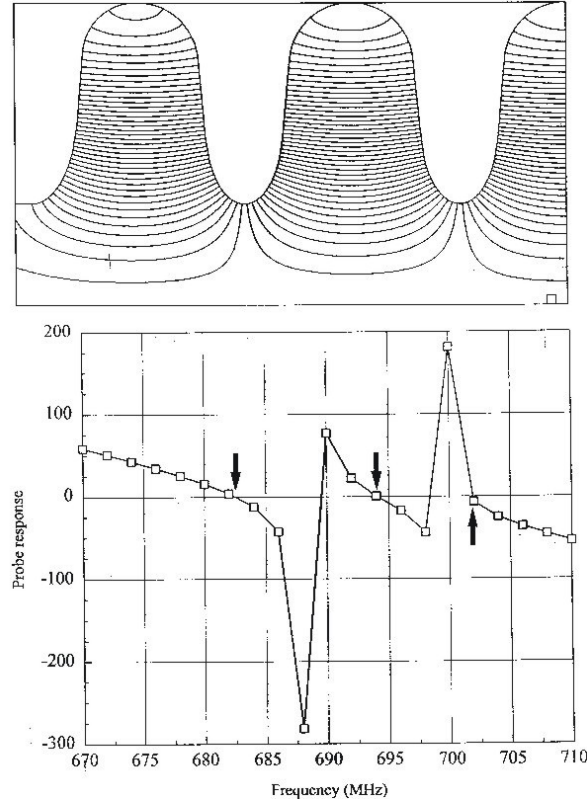
Figure 41: Resonant modes in a proton accelerator structure, coupled superconducting cavities. a) Simulation geometry for half of a 5-cavity assembly. Symmetry boundary on the right-hand side, drive current region at the bottom-right. Electric field lines for the \pi -mode. b) Scan of probe output as a function of frequency – arrows show the locations of the 0, \pi/2 and \pi modes.
