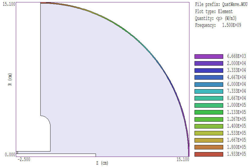
Figure 25: Geometry of the QUATWAVE example. The air volume is shaded in blue. The absorption layer is color-coded by time-averaged power density to illustrate the radiation pattern.
