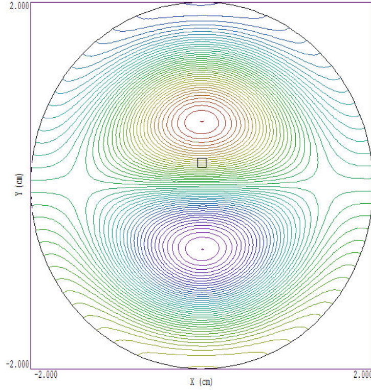
Figure 17: Electric field lines, TE_{02} mode at cutoff in a circular waveguide of radius R = 2.0 cm.
