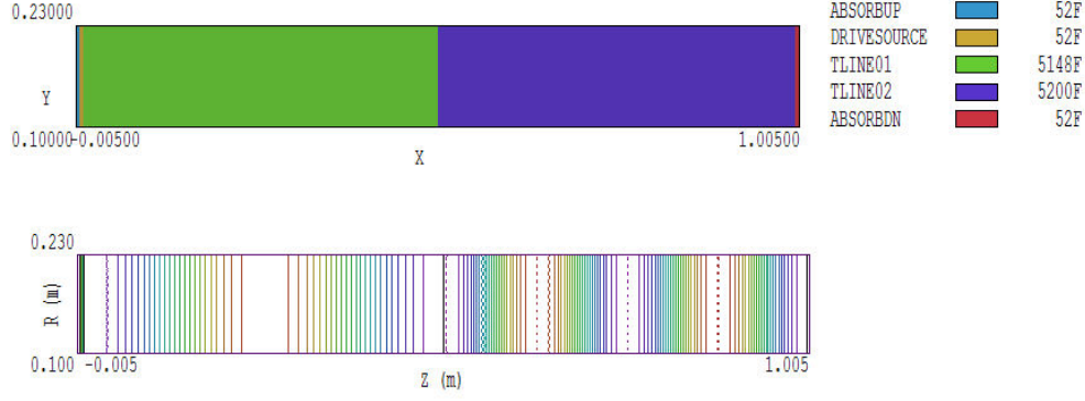
Figure 21: Example TCONNECT. a) Geometry showing region divisions. b) Electric field lines in a line with \epsilon_r = 1.0 in the left volume and \epsilon_r = 4.0 on the right.
