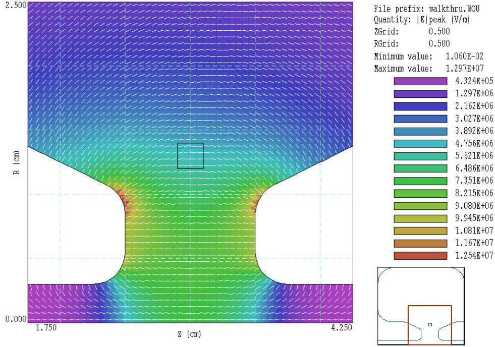
Figure 10: Electric field magnitude and direction near the deceleration gap, values from the normalized example WALKTHRUNORM .
