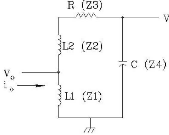
Figure 37: Driven LCR resonant circuit.
