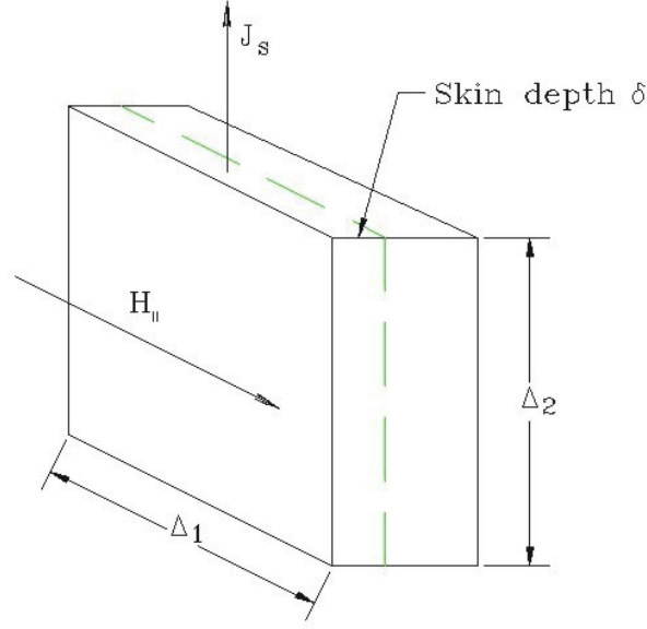
Figure 42: RF power loss by currents driven in a metal wall.
