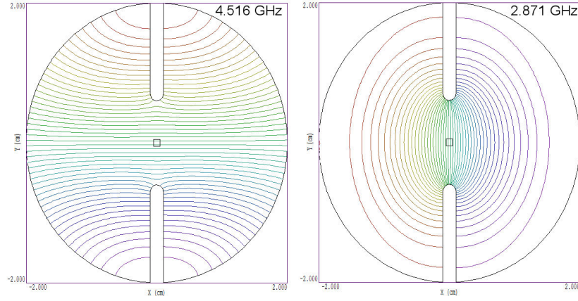
Figure 18: Electric field lines in a modified circular waveguide, with fins to shift the frequency of the TE_{01} mode, depending on the polarization of electric fields.
