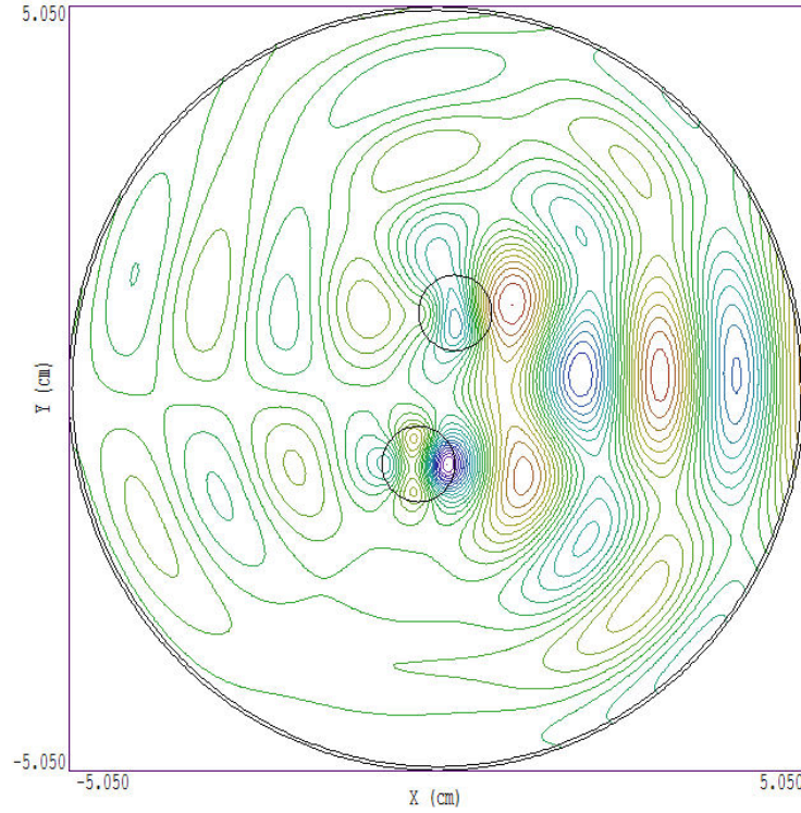
Figure 30: Example DOUBLEBAR, \mathbf{H} lines of the scattered field.
